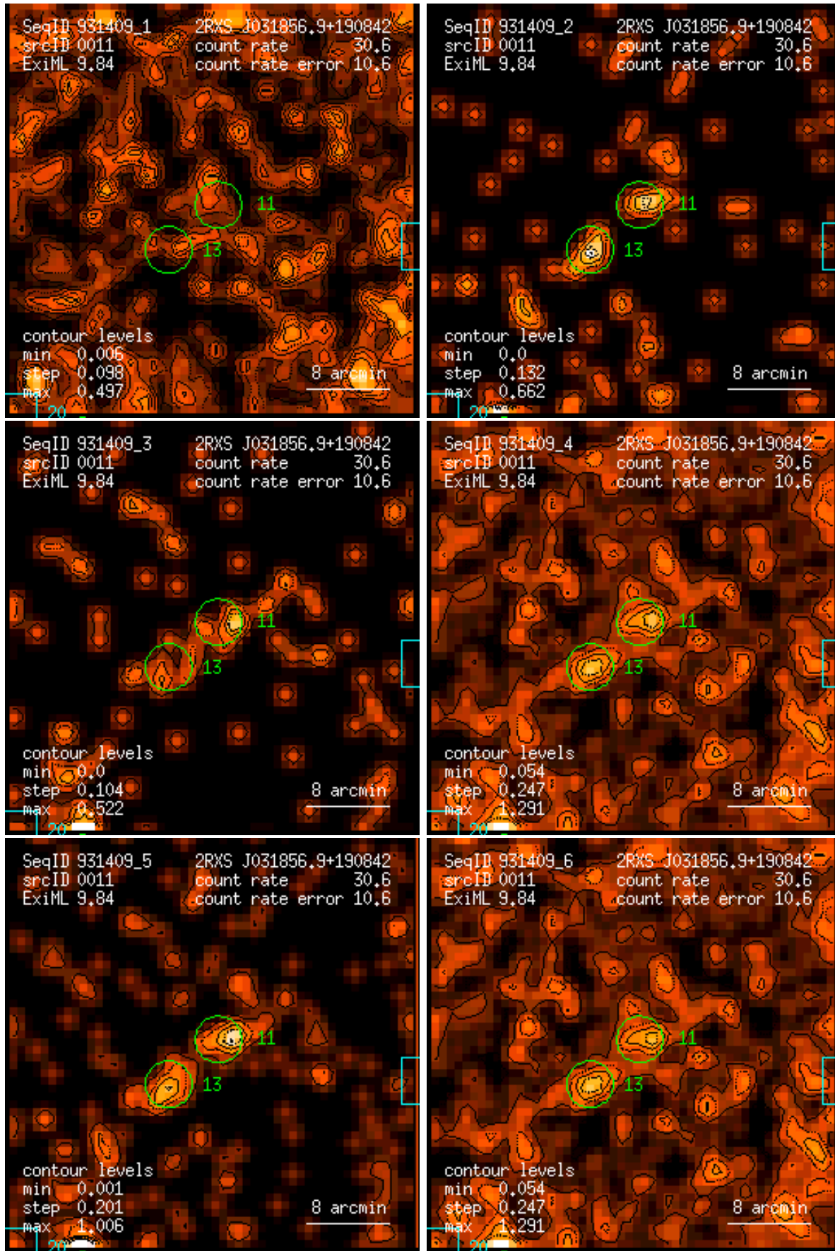
Figure 11: RASS 931409: detection 0011: band rate images, Gaussian filter: (1) PSPC channels 11 – 41, (2) 52 – 90, (3) 91 – 201, (4) 11 – 235, (5) 52 – 201, (6) 11 – 201. Broad band rates in counts/ks. Band rate contour levels in counts/ks/arcmin 2 .
