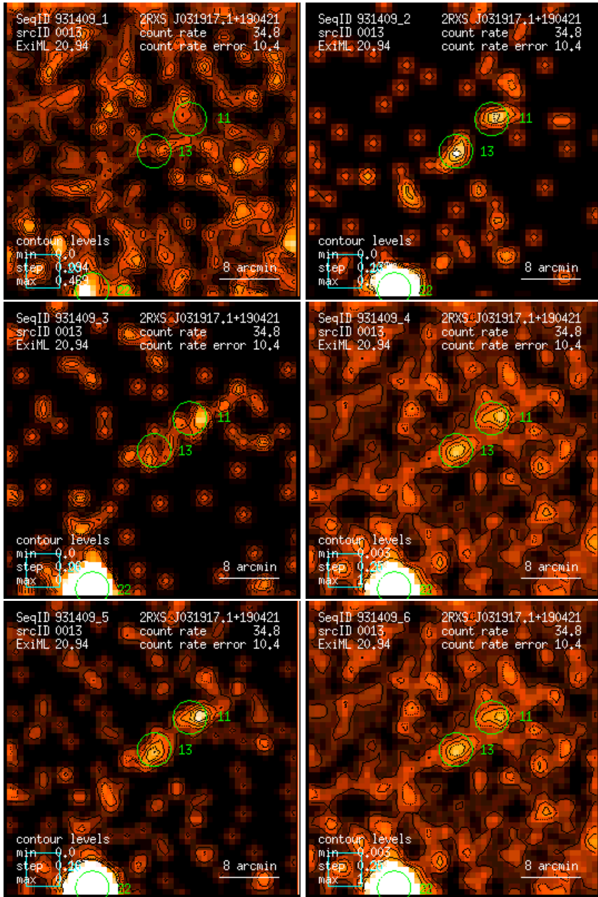
Figure 13: RASS 931409: detection 0013: band rate images, Gaussian filter: (1) PSPC channels 11 – 41, (2) 52 – 90, (3) 91 – 201, (4) 11 – 235, (5) 52 – 201, (6) 11 – 201. Broad band rates in counts/ks. Band rate contour levels in counts/ks/arcmin 2 .
