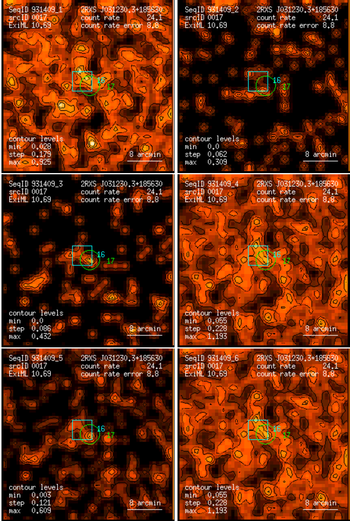
Figure 17: RASS 931409: detection 0017: band rate images, Gaussian filter: (1) PSPC channels 11 – 41, (2) 52 – 90, (3) 91 – 201, (4) 11 – 235, (5) 52 – 201, (6) 11 – 201. Broad band rates in counts/ks. Band rate contour levels in counts/ks/arcmin 2 .
