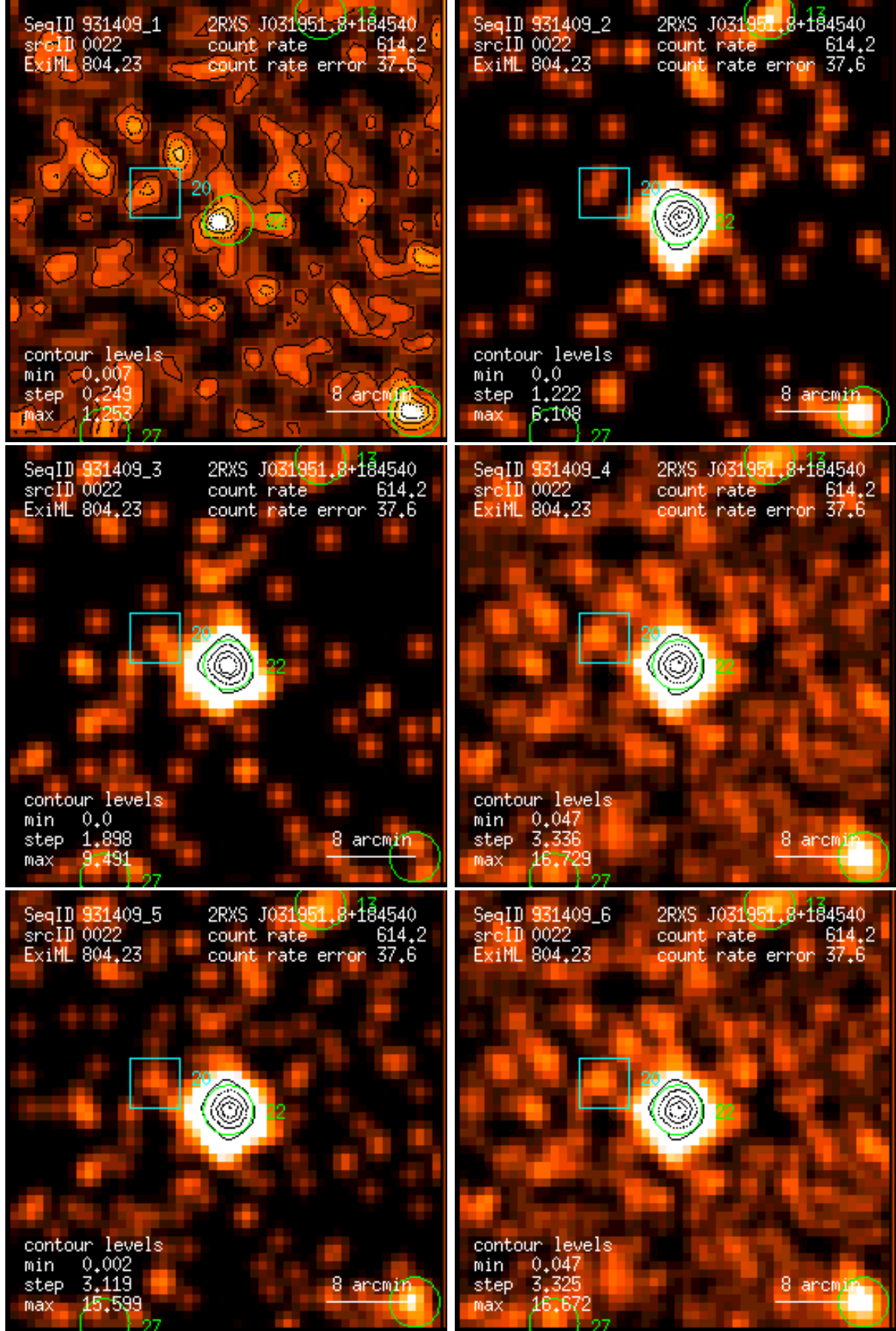
Figure 22: RASS 931409: detection 0022: band rate images, Gaussian filter: (1) PSPC channels 11 – 41, (2) 52 – 90, (3) 91 – 201, (4) 11 – 235, (5) 52 – 201, (6) 11 – 201. Broad band rates in counts/ks. Band rate contour levels in counts/ks/arcmin 2 .
