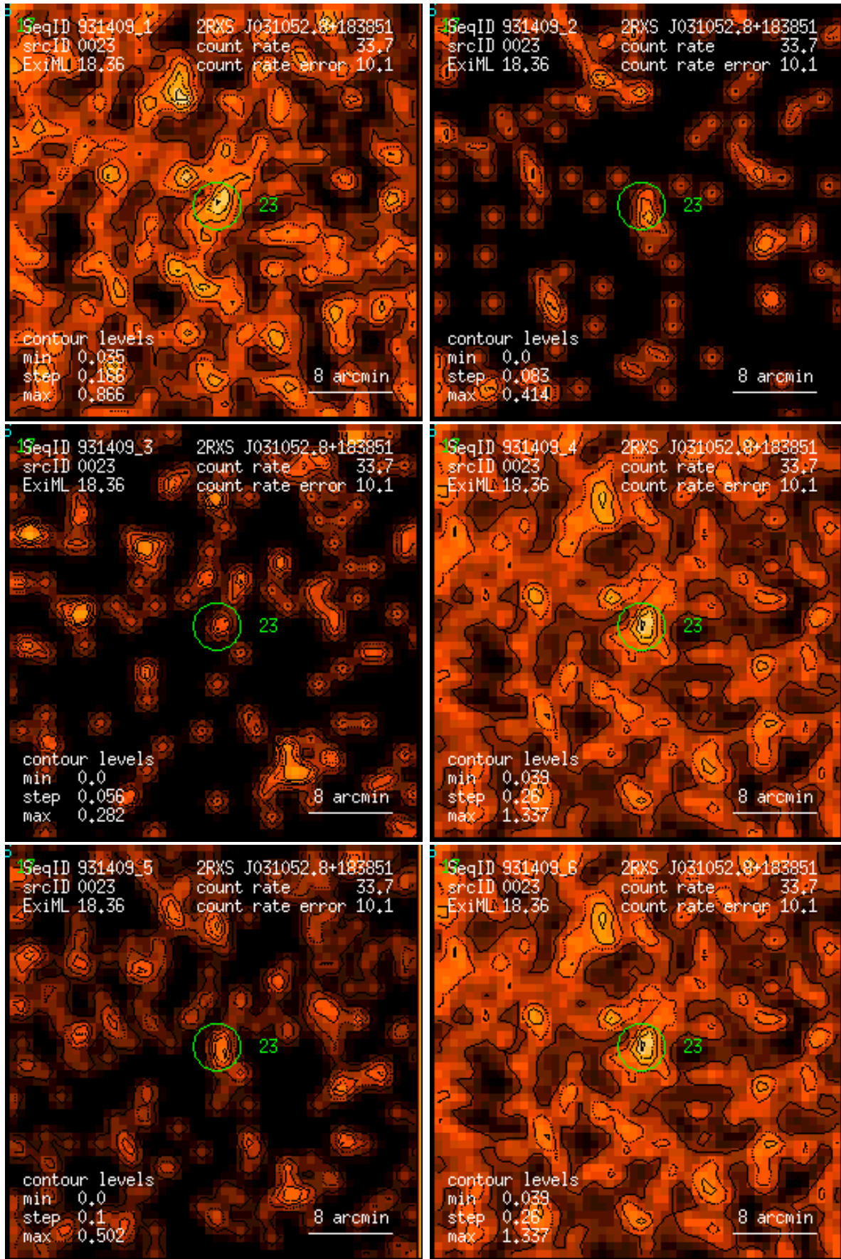
Figure 23: RASS 931409: detection 0023: band rate images, Gaussian filter: (1) PSPC channels 11 – 41, (2) 52 – 90, (3) 91 – 201, (4) 11 – 235, (5) 52 – 201, (6) 11 – 201. Broad band rates in counts/ks. Band rate contour levels in counts/ks/arcmin 2 .
