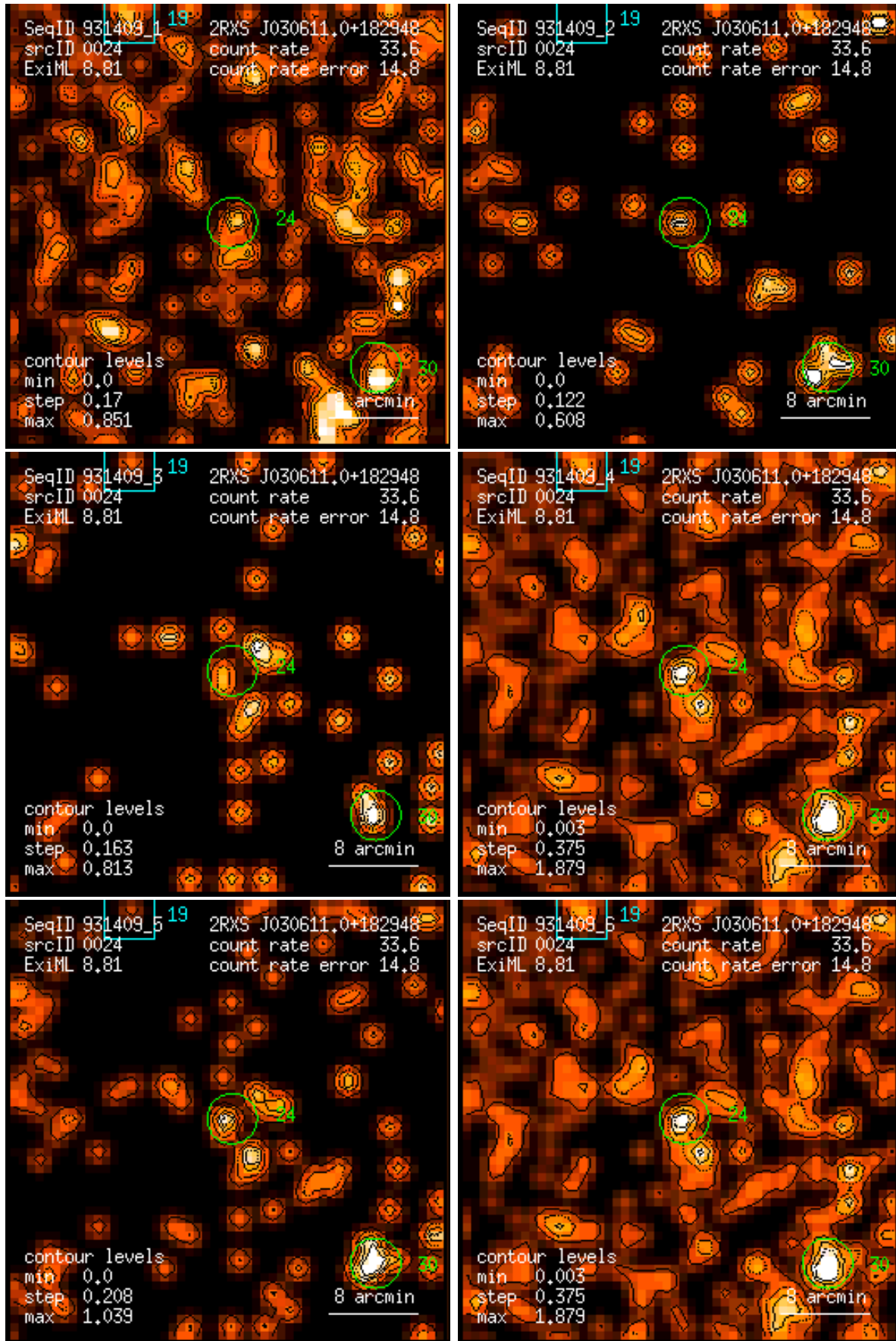
Figure 24: RASS 931409: detection 0024: band rate images, Gaussian filter: (1) PSPC channels 11 – 41, (2) 52 – 90, (3) 91 – 201, (4) 11 – 235, (5) 52 – 201, (6) 11 – 201. Broad band rates in counts/ks. Band rate contour levels in counts/ks/arcmin 2 .
