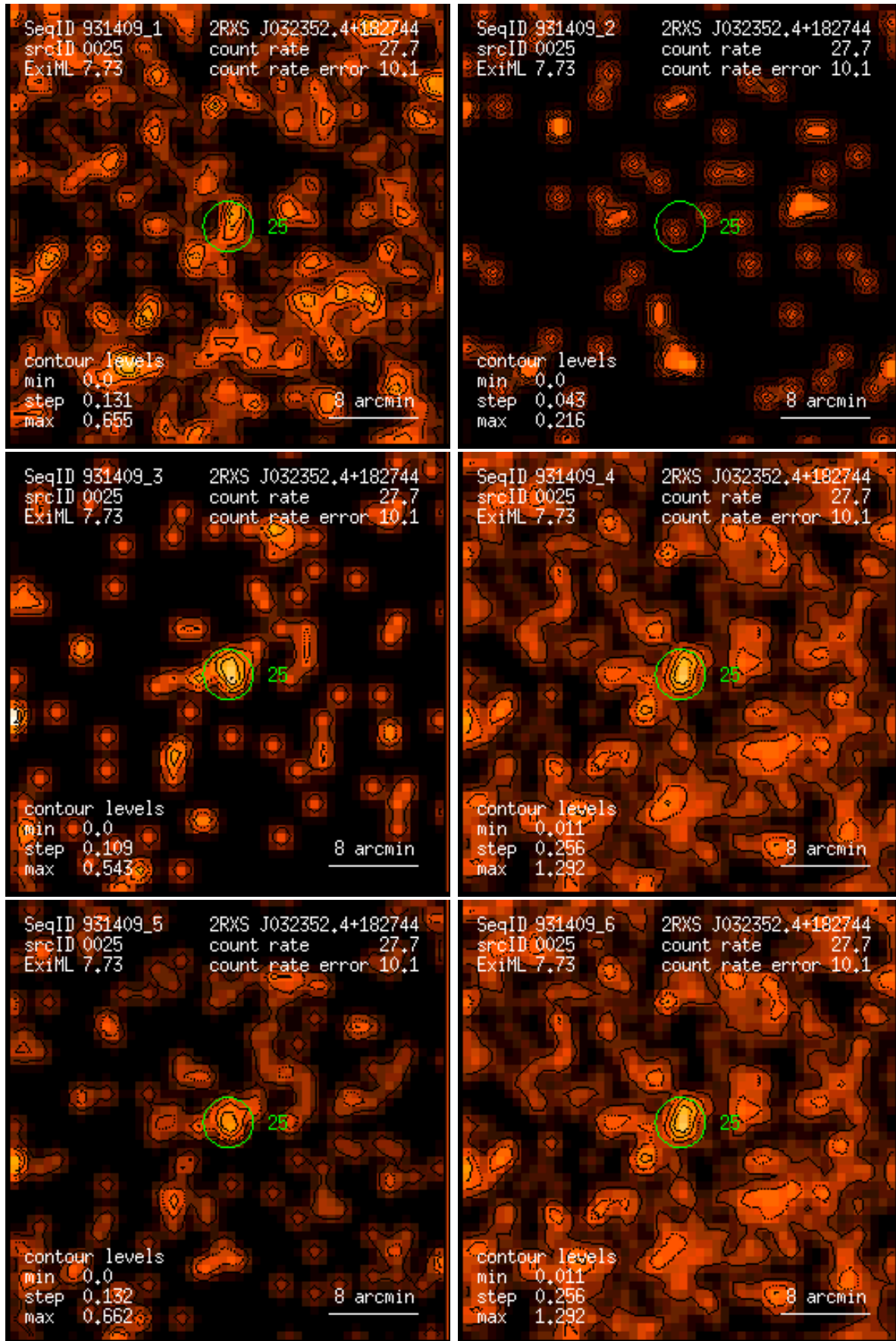
Figure 25: RASS 931409: detection 0025: band rate images, Gaussian filter: (1) PSPC channels 11 – 41, (2) 52 – 90, (3) 91 – 201, (4) 11 – 235, (5) 52 – 201, (6) 11 – 201. Broad band rates in counts/ks. Band rate contour levels in counts/ks/arcmin 2 .
