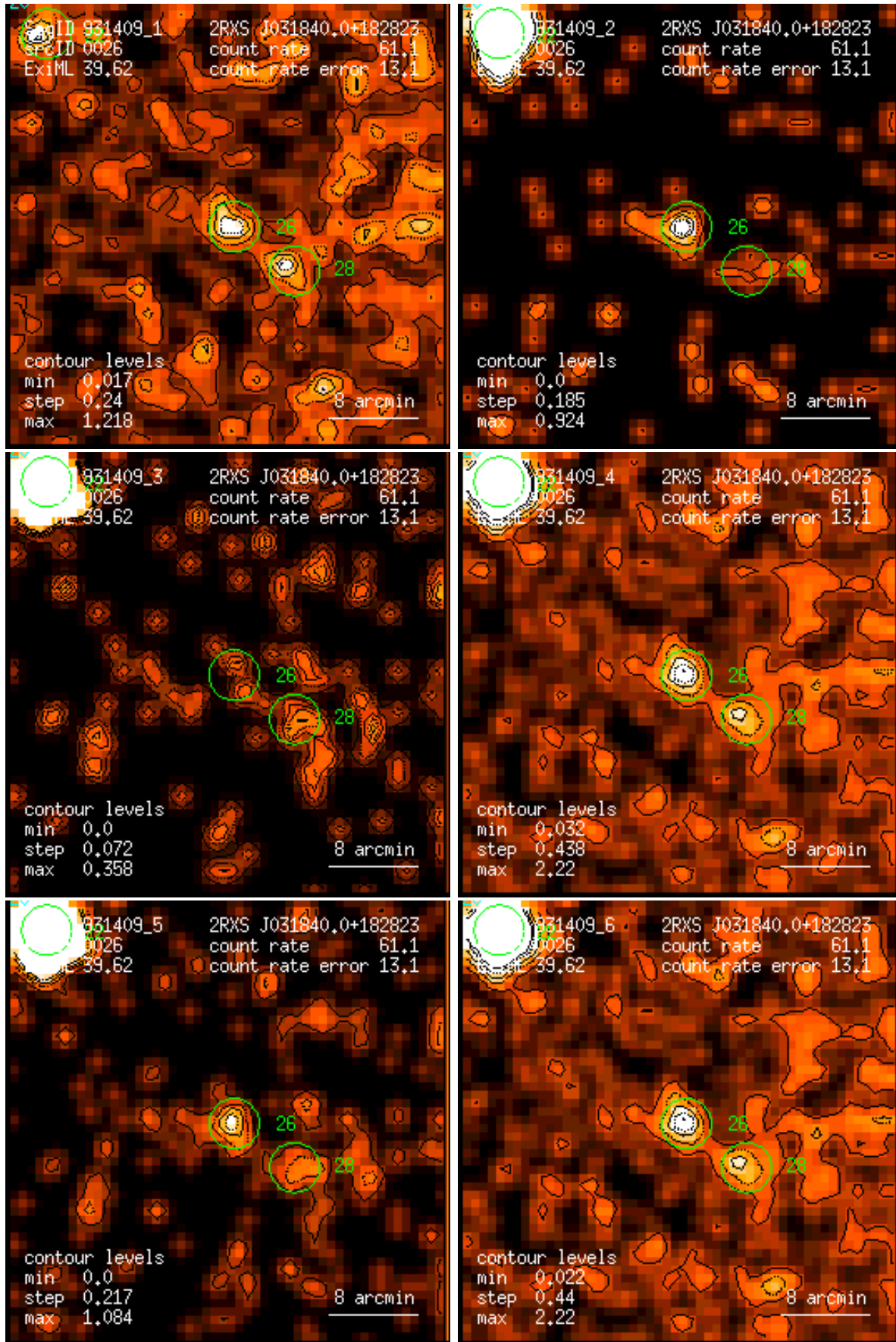
Figure 26: RASS 931409: detection 0026: band rate images, Gaussian filter: (1) PSPC channels 11 – 41, (2) 52 – 90, (3) 91 – 201, (4) 11 – 235, (5) 52 – 201, (6) 11 – 201. Broad band rates in counts/ks. Band rate contour levels in counts/ks/arcmin 2 .
