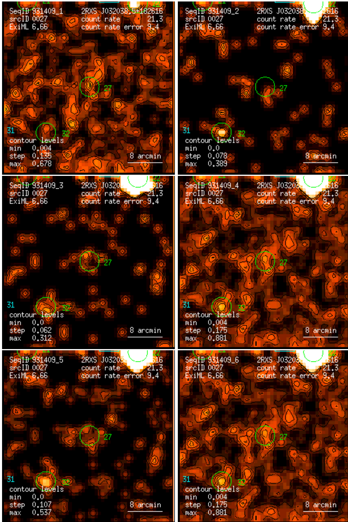
Figure 27: RASS 931409: detection 0027: band rate images, Gaussian filter: (1) PSPC channels 11 – 41, (2) 52 – 90, (3) 91 – 201, (4) 11 – 235, (5) 52 – 201, (6) 11 – 201. Broad band rates in counts/ks. Band rate contour levels in counts/ks/arcmin 2 .
