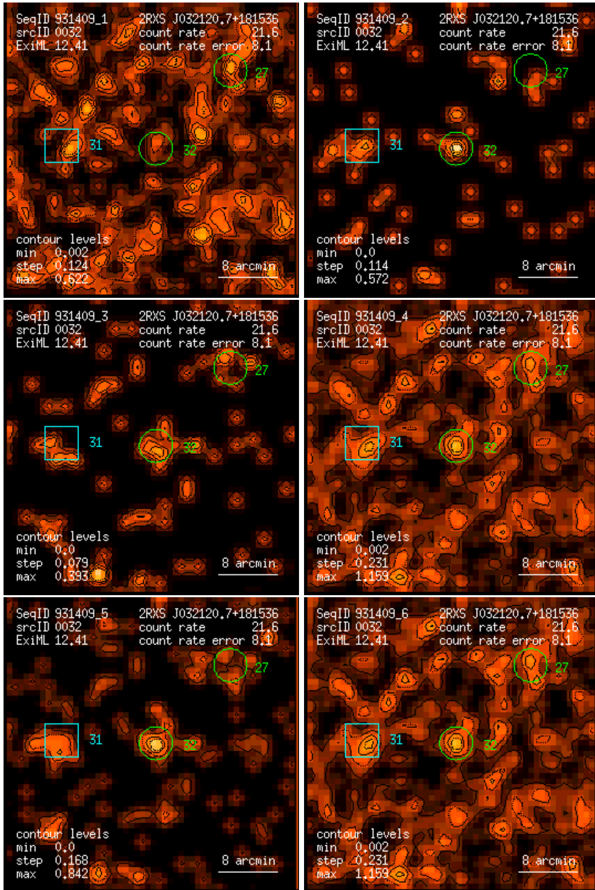
Figure 32: RASS 931409: detection 0032: band rate images, Gaussian filter: (1) PSPC channels 11 – 41, (2) 52 – 90, (3) 91 – 201, (4) 11 – 235, (5) 52 – 201, (6) 11 – 201. Broad band rates in counts/ks. Band rate contour levels in counts/ks/arcmin 2 .
