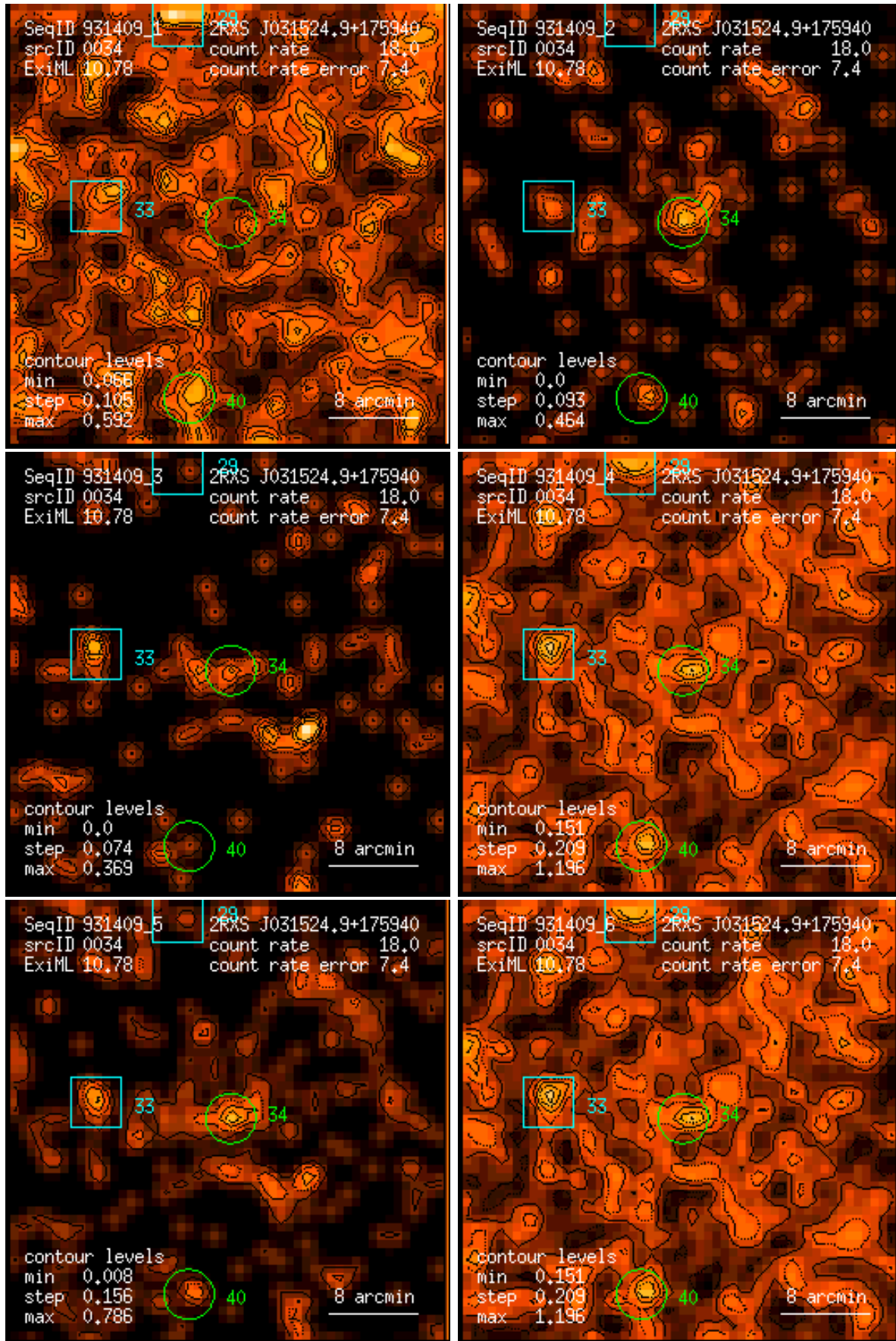
Figure 34: RASS 931409: detection 0034: band rate images, Gaussian filter: (1) PSPC channels 11 – 41, (2) 52 – 90, (3) 91 – 201, (4) 11 – 235, (5) 52 – 201, (6) 11 – 201. Broad band rates in counts/ks. Band rate contour levels in counts/ks/arcmin 2 .
