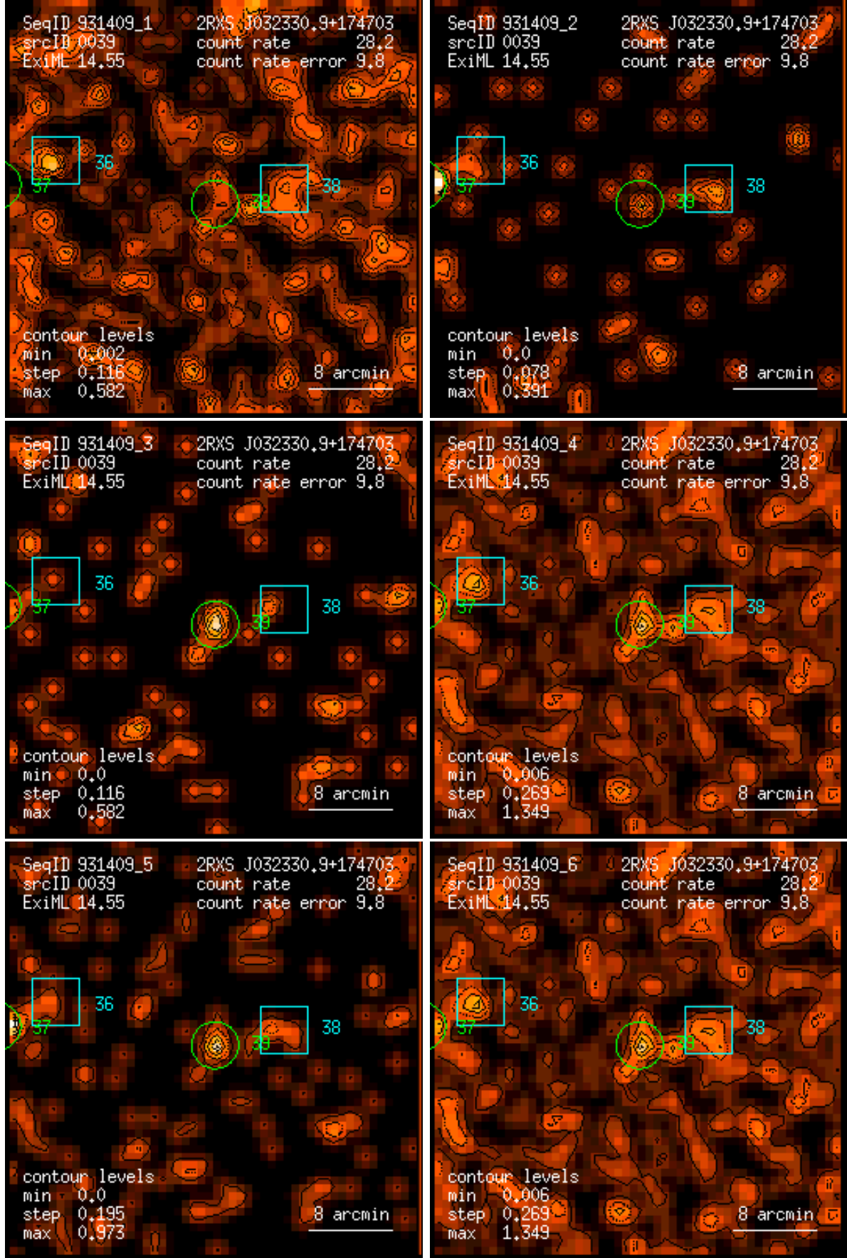
Figure 39: RASS 931409: detection 0039: band rate images, Gaussian filter: (1) PSPC channels 11 – 41, (2) 52 – 90, (3) 91 – 201, (4) 11 – 235, (5) 52 – 201, (6) 11 – 201. Broad band rates in counts/ks. Band rate contour levels in counts/ks/arcmin 2 .
