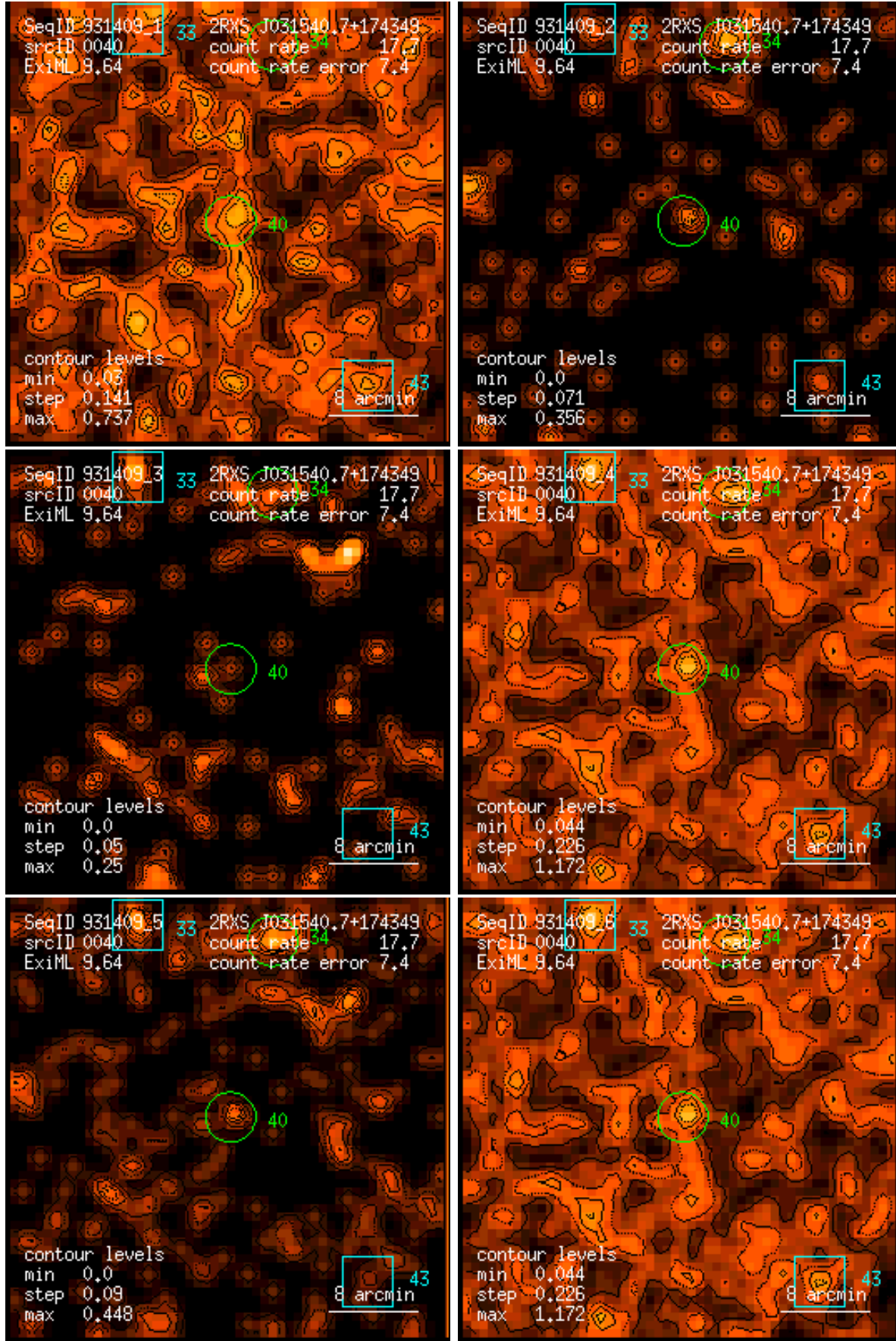
Figure 40: RASS 931409: detection 0040: band rate images, Gaussian filter: (1) PSPC channels 11 – 41, (2) 52 – 90, (3) 91 – 201, (4) 11 – 235, (5) 52 – 201, (6) 11 – 201. Broad band rates in counts/ks. Band rate contour levels in counts/ks/arcmin 2 .
