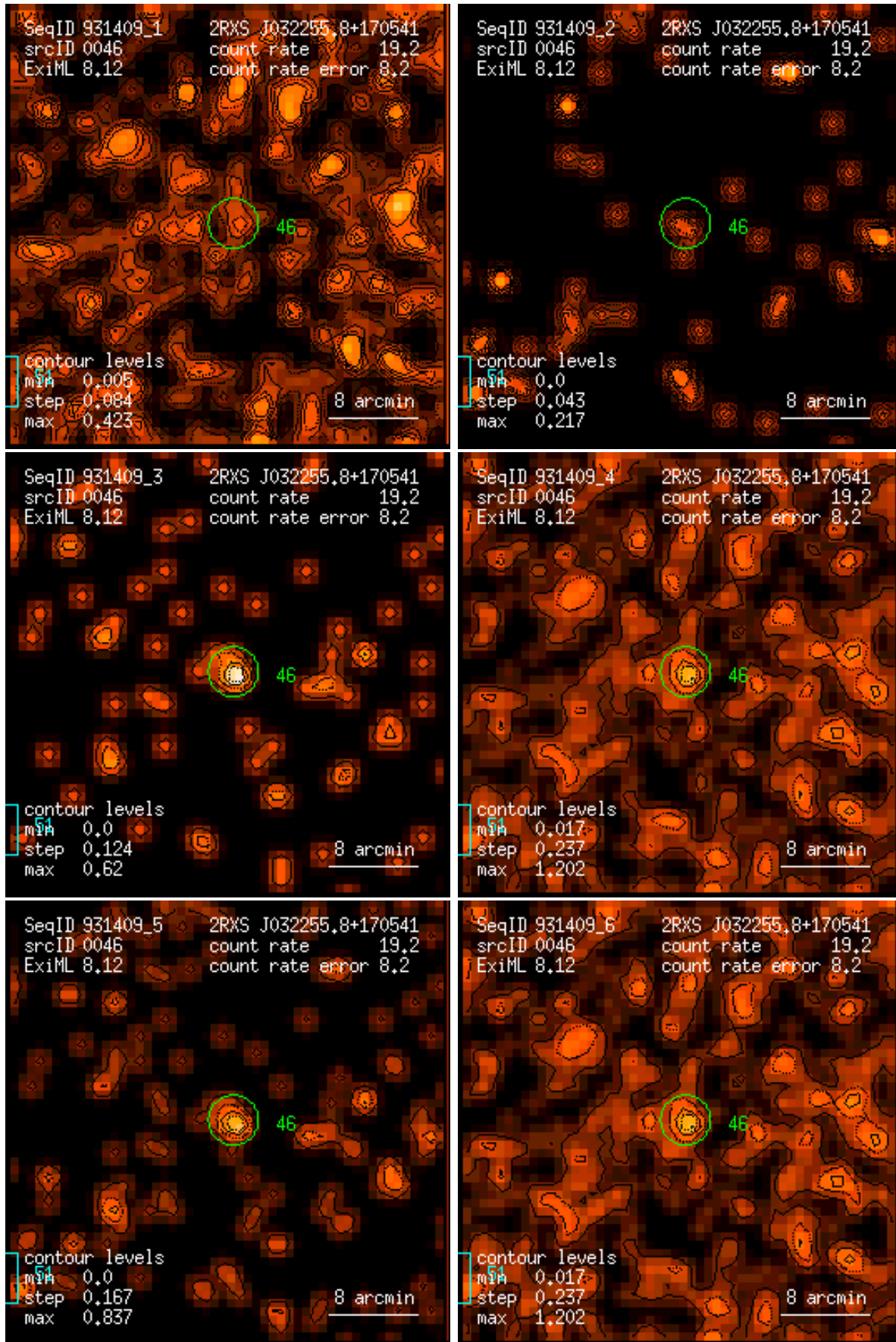
Figure 46: RASS 931409: detection 0046: band rate images, Gaussian filter: (1) PSPC channels 11 – 41, (2) 52 – 90, (3) 91 – 201, (4) 11 – 235, (5) 52 – 201, (6) 11 – 201. Broad band rates in counts/ks. Band rate contour levels in counts/ks/arcmin 2 .
