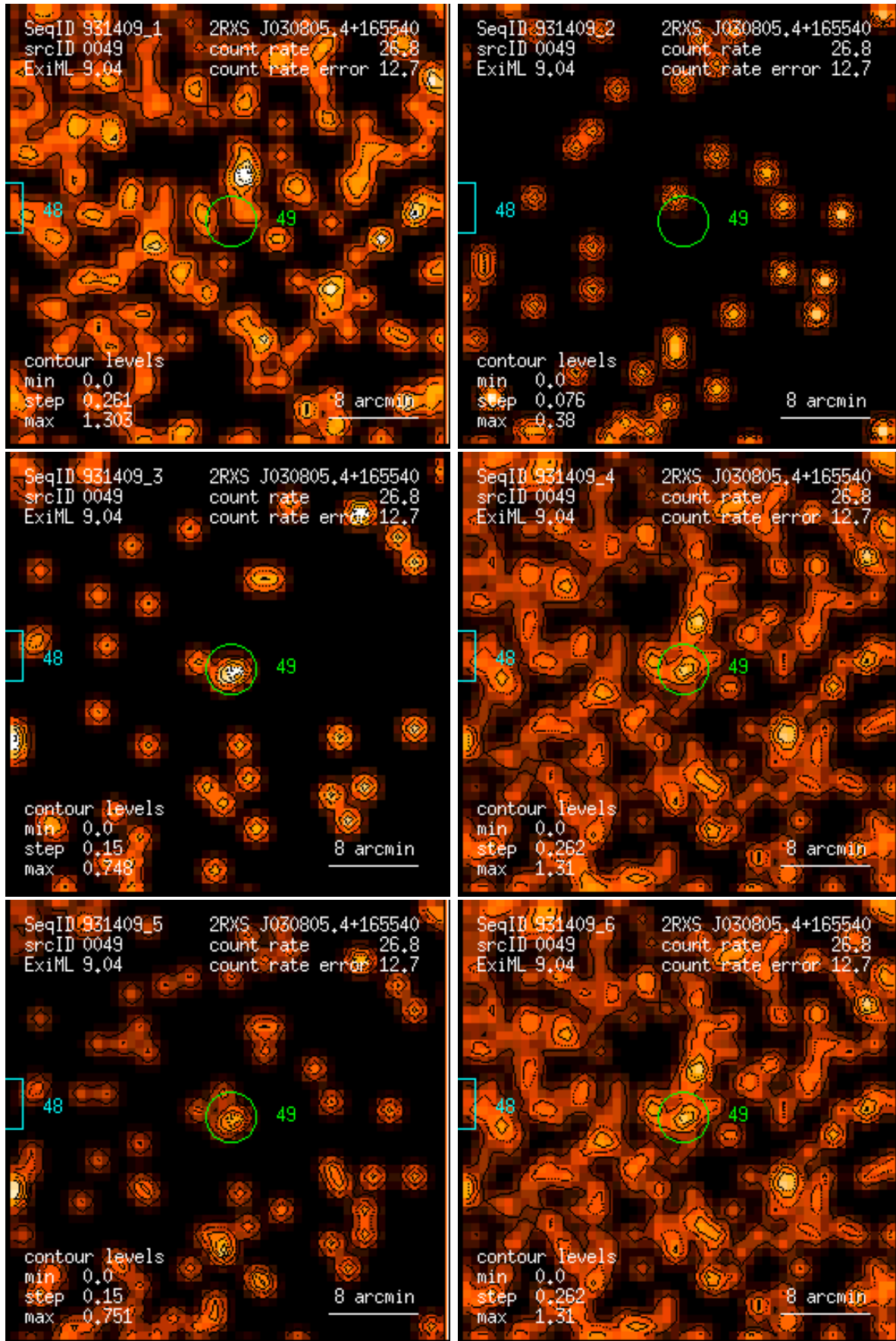
Figure 49: RASS 931409: detection 0049: band rate images, Gaussian filter: (1) PSPC channels 11 – 41, (2) 52 – 90, (3) 91 – 201, (4) 11 – 235, (5) 52 – 201, (6) 11 – 201. Broad band rates in counts/ks. Band rate contour levels in counts/ks/arcmin 2 .
