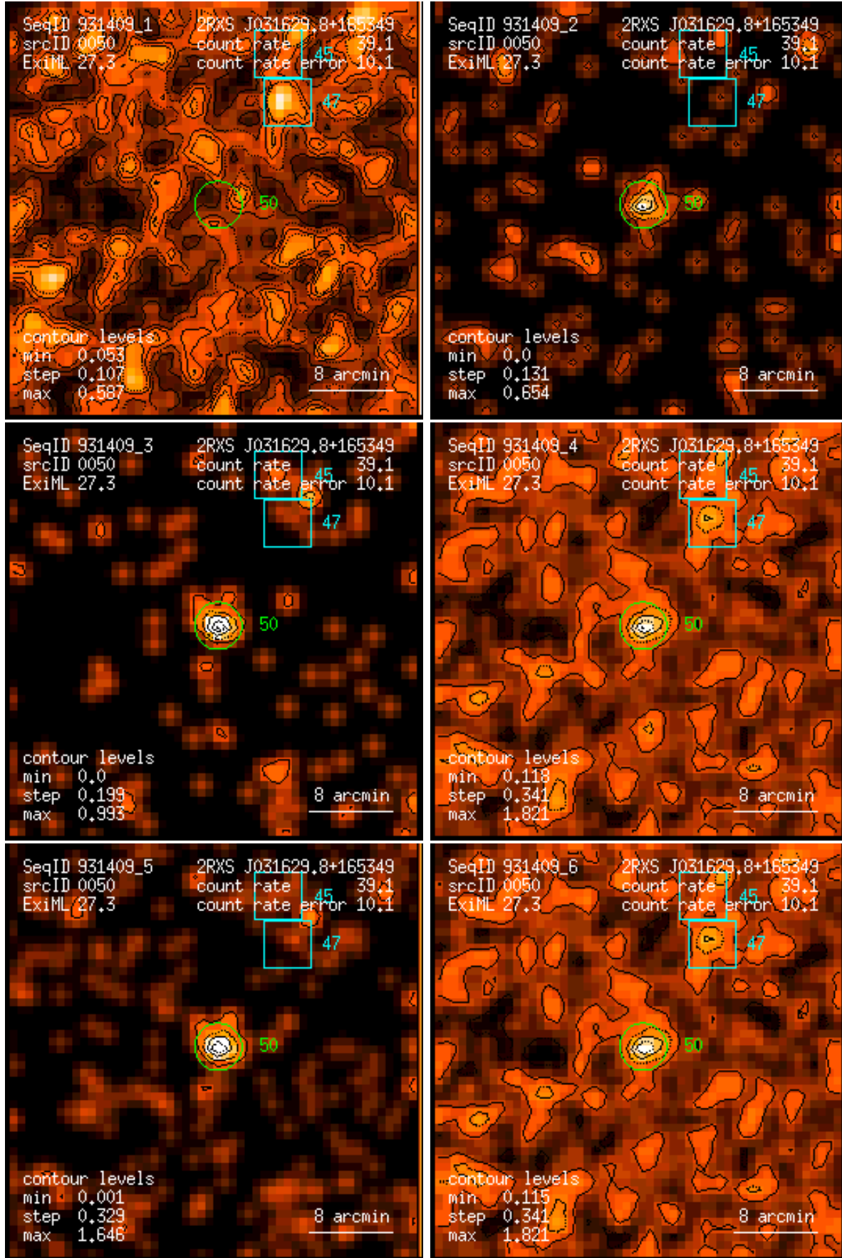
Figure 50: RASS 931409: detection 0050: band rate images, Gaussian filter: (1) PSPC channels 11 – 41, (2) 52 – 90, (3) 91 – 201, (4) 11 – 235, (5) 52 – 201, (6) 11 – 201. Broad band rates in counts/ks. Band rate contour levels in counts/ks/arcmin 2 .
