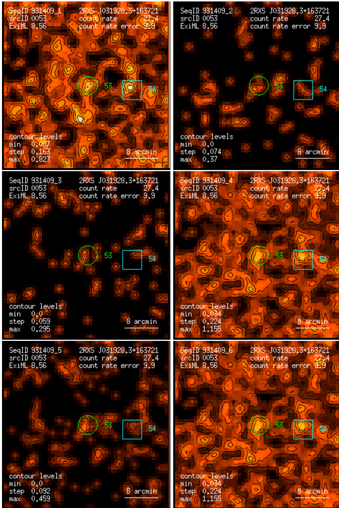
Figure 53: RASS 931409: detection 0053: band rate images, Gaussian filter: (1) PSPC channels 11 – 41, (2) 52 – 90, (3) 91 – 201, (4) 11 – 235, (5) 52 – 201, (6) 11 – 201. Broad band rates in counts/ks. Band rate contour levels in counts/ks/arcmin 2 .
