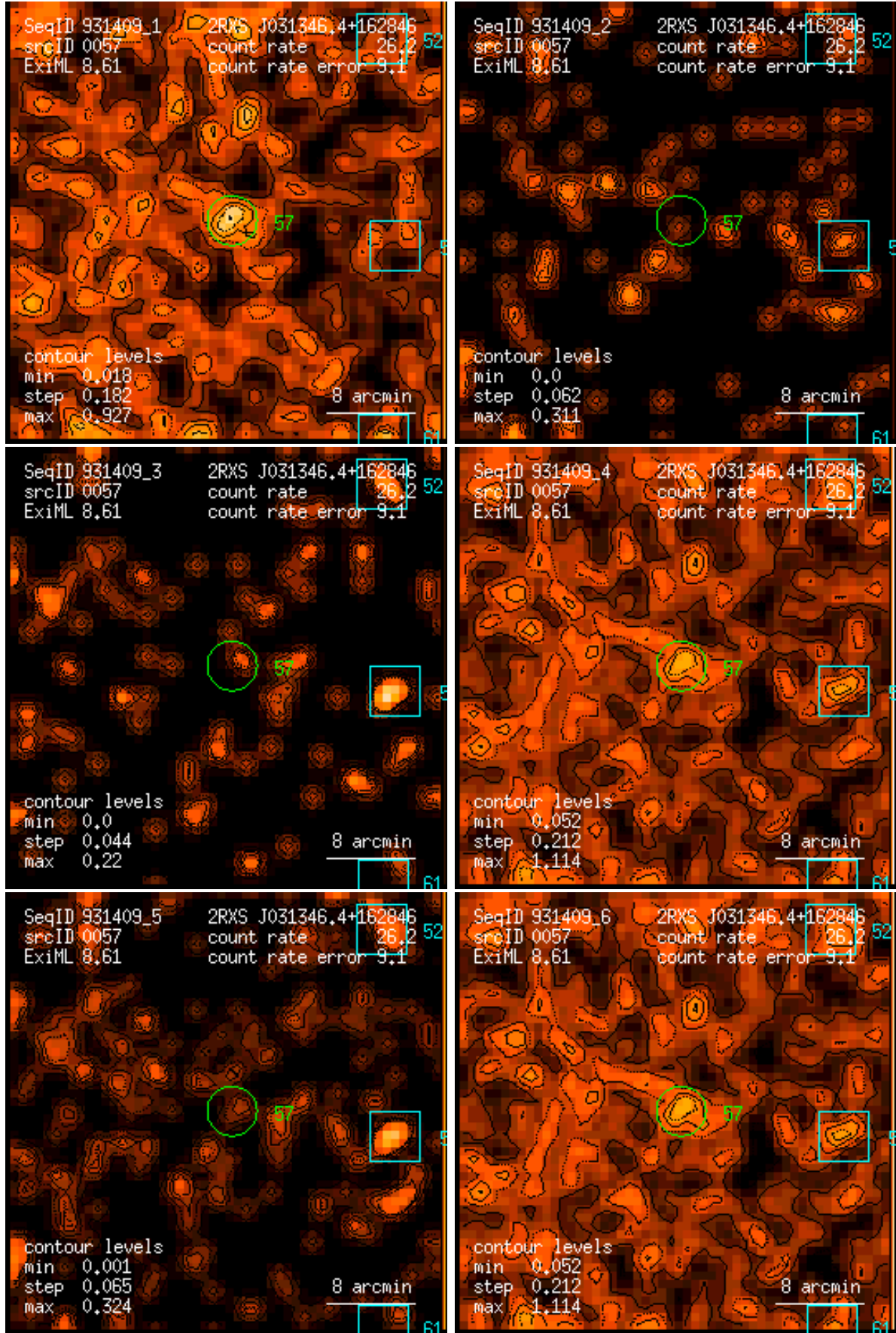
Figure 57: RASS 931409: detection 0057: band rate images, Gaussian filter: (1) PSPC channels 11 – 41, (2) 52 – 90, (3) 91 – 201, (4) 11 – 235, (5) 52 – 201, (6) 11 – 201. Broad band rates in counts/ks. Band rate contour levels in counts/ks/arcmin 2 .
