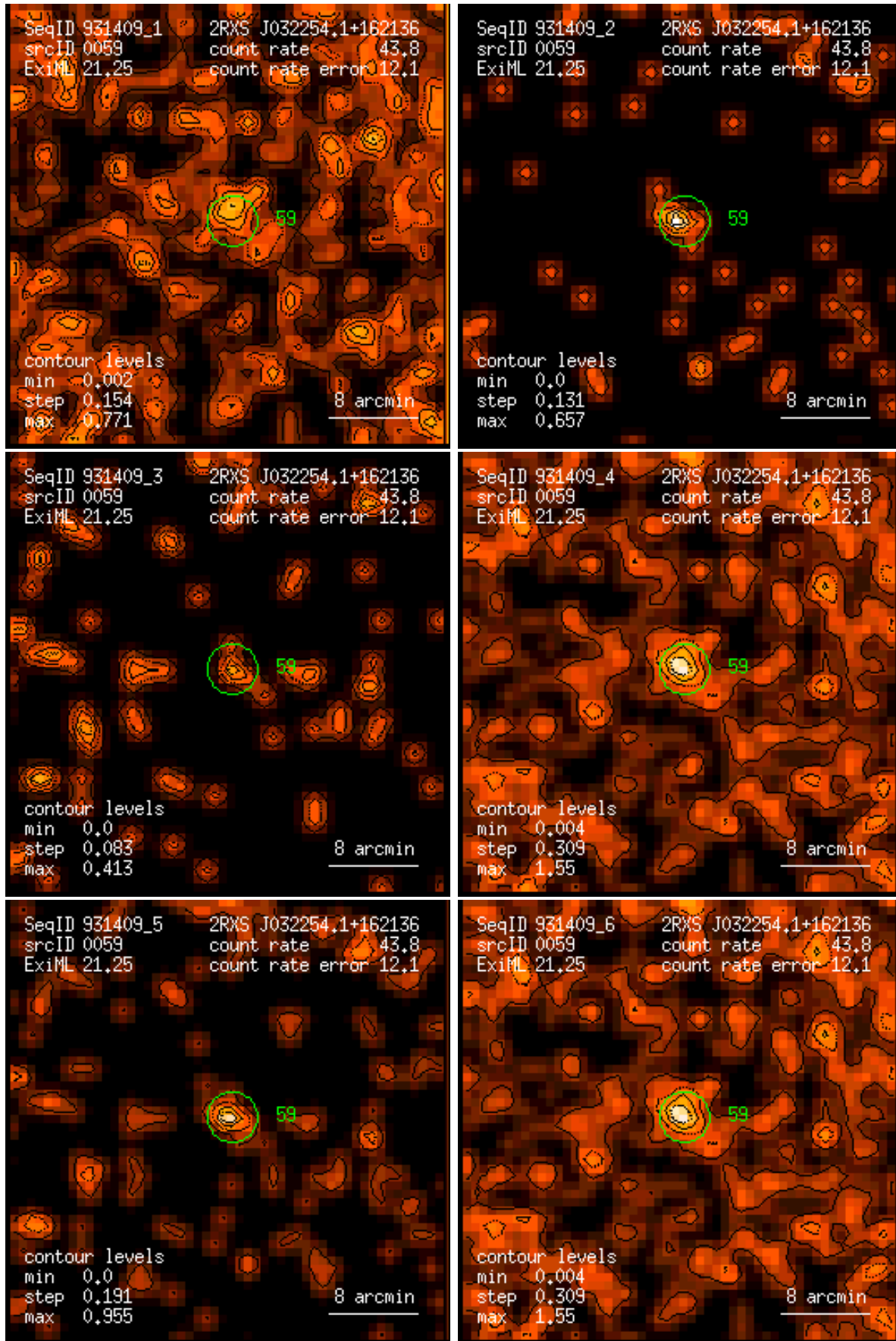
Figure 59: RASS 931409: detection 0059: band rate images, Gaussian filter: (1) PSPC channels 11 – 41, (2) 52 – 90, (3) 91 – 201, (4) 11 – 235, (5) 52 – 201, (6) 11 – 201. Broad band rates in counts/ks. Band rate contour levels in counts/ks/arcmin 2 .
