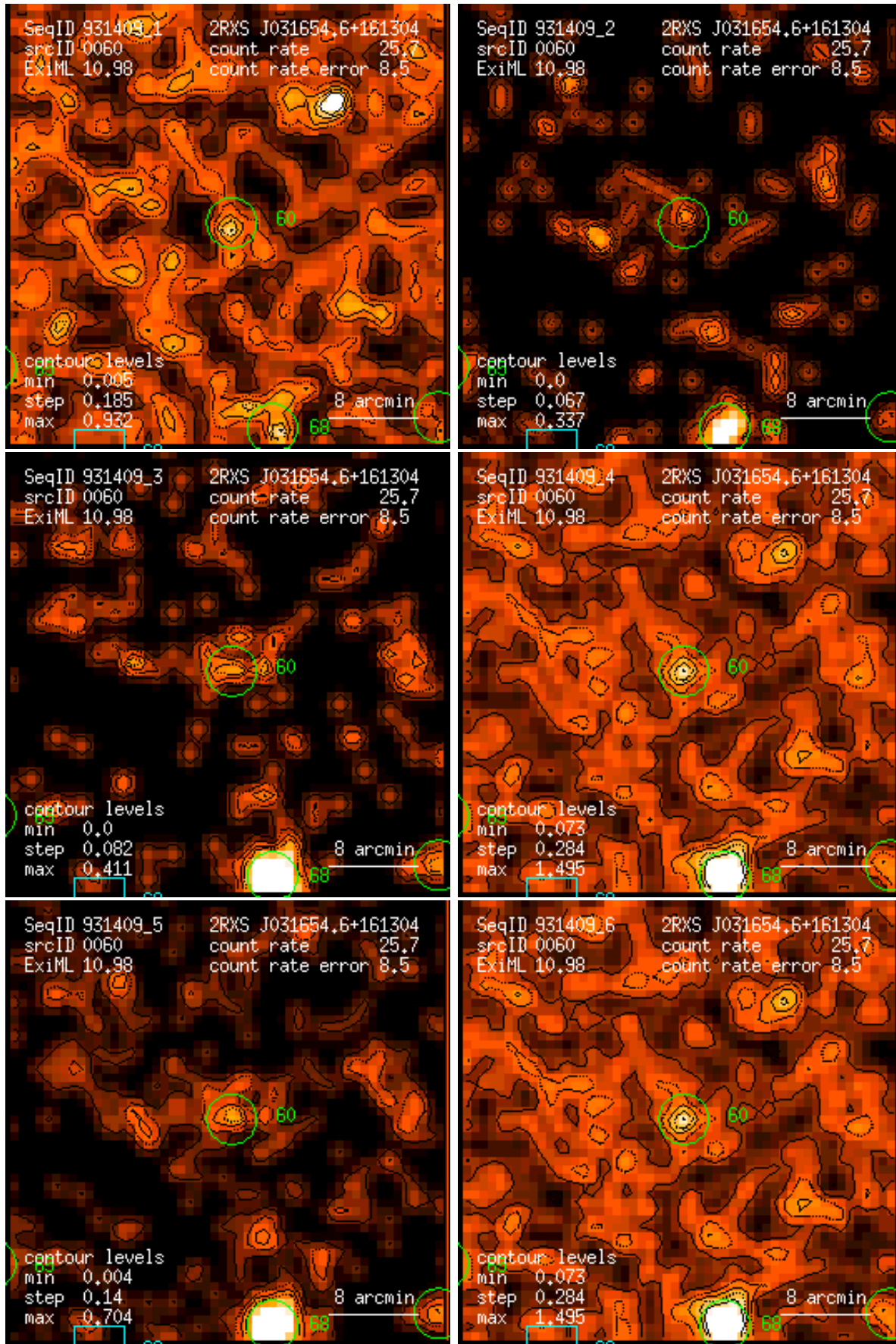
Figure 60: RASS 931409: detection 0060: band rate images, Gaussian filter: (1) PSPC channels 11 – 41, (2) 52 – 90, (3) 91 – 201, (4) 11 – 235, (5) 52 – 201, (6) 11 – 201. Broad band rates in counts/ks. Band rate contour levels in counts/ks/arcmin 2 .
