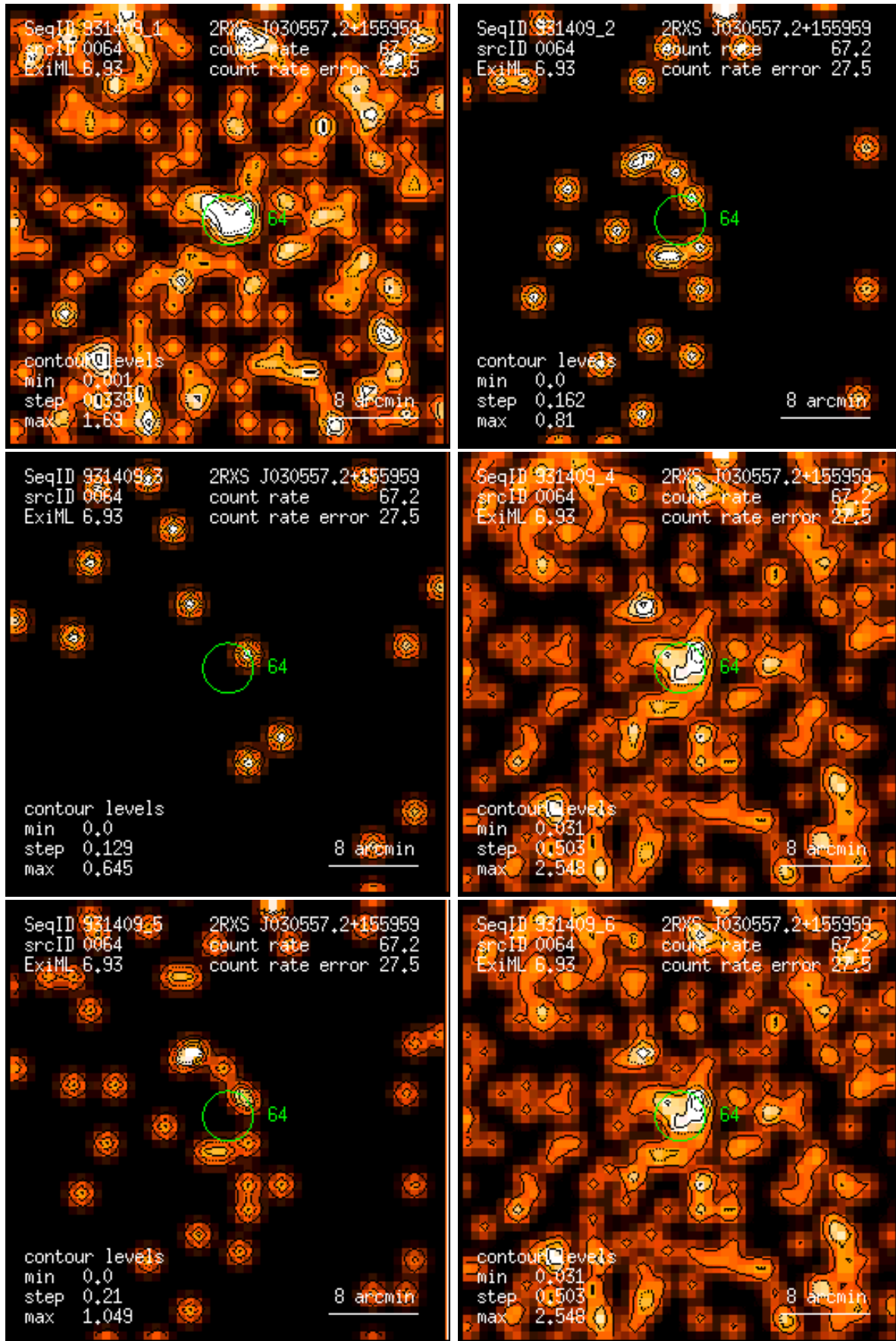
Figure 64: RASS 931409: detection 0064: band rate images, Gaussian filter: (1) PSPC channels 11 – 41, (2) 52 – 90, (3) 91 – 201, (4) 11 – 235, (5) 52 – 201, (6) 11 – 201. Broad band rates in counts/ks. Band rate contour levels in counts/ks/arcmin 2 .
