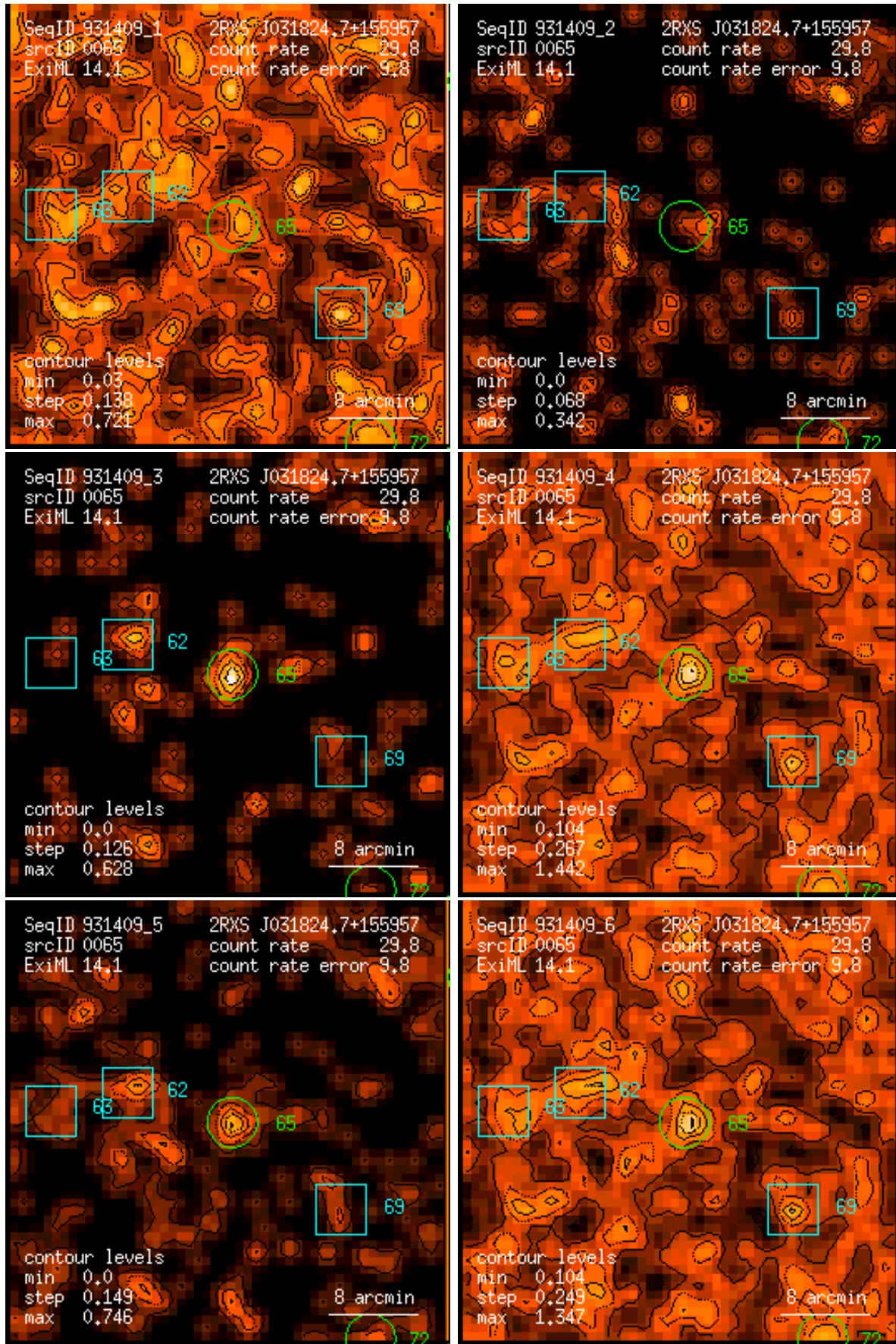
Figure 65: RASS 931409: detection 0065: band rate images, Gaussian filter: (1) PSPC channels 11 – 41, (2) 52 – 90, (3) 91 – 201, (4) 11 – 235, (5) 52 – 201, (6) 11 – 201. Broad band rates in counts/ks. Band rate contour levels in counts/ks/arcmin 2 .
