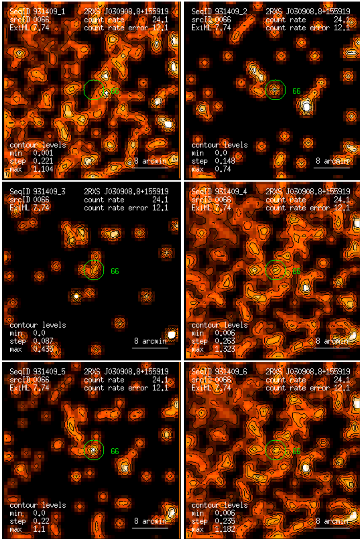
Figure 66: RASS 931409: detection 0066: band rate images, Gaussian filter: (1) PSPC channels 11 – 41, (2) 52 – 90, (3) 91 – 201, (4) 11 – 235, (5) 52 – 201, (6) 11 – 201. Broad band rates in counts/ks. Band rate contour levels in counts/ks/arcmin 2 .
