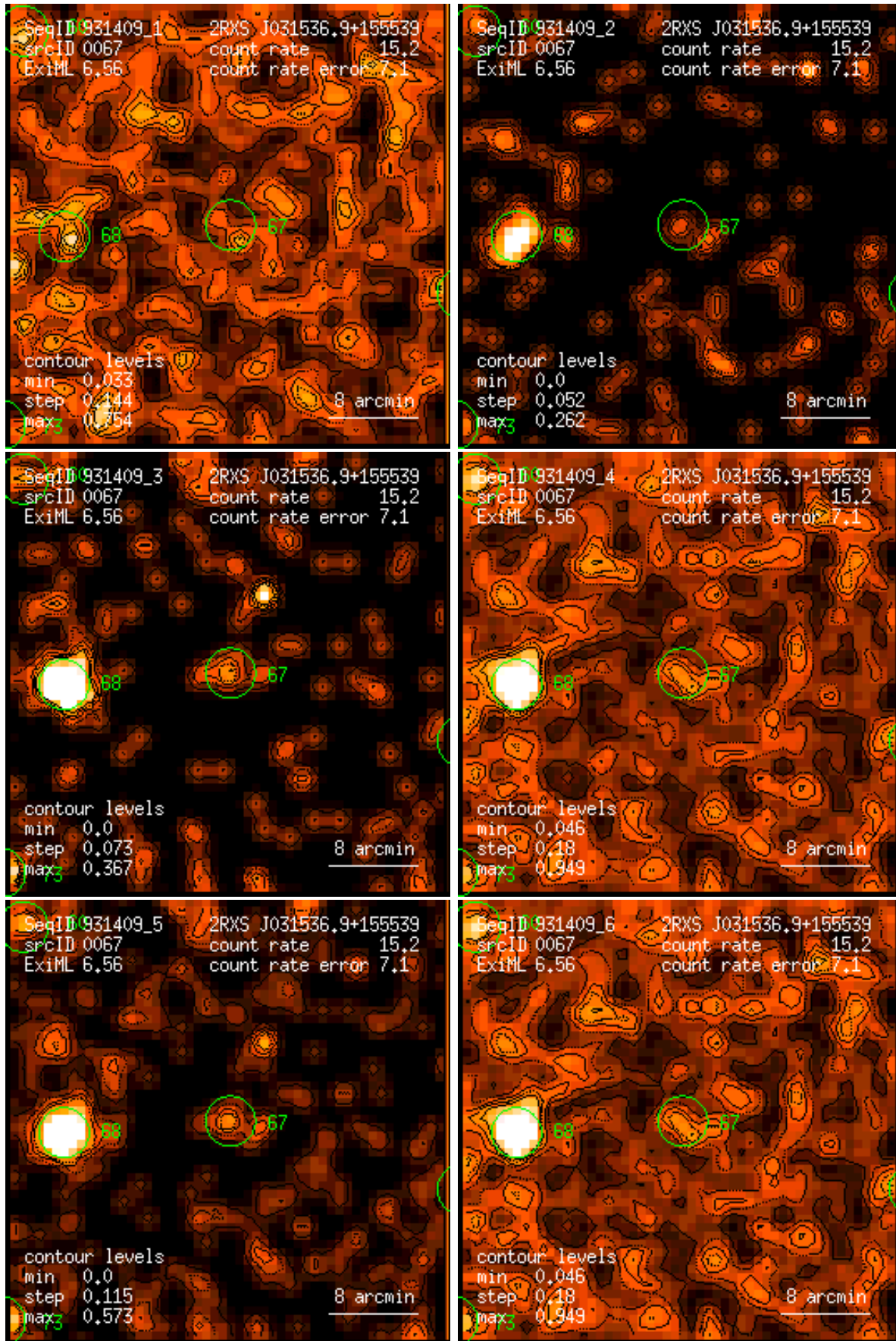
Figure 67: RASS 931409: detection 0067: band rate images, Gaussian filter: (1) PSPC channels 11 – 41, (2) 52 – 90, (3) 91 – 201, (4) 11 – 235, (5) 52 – 201, (6) 11 – 201. Broad band rates in counts/ks. Band rate contour levels in counts/ks/arcmin 2 .
