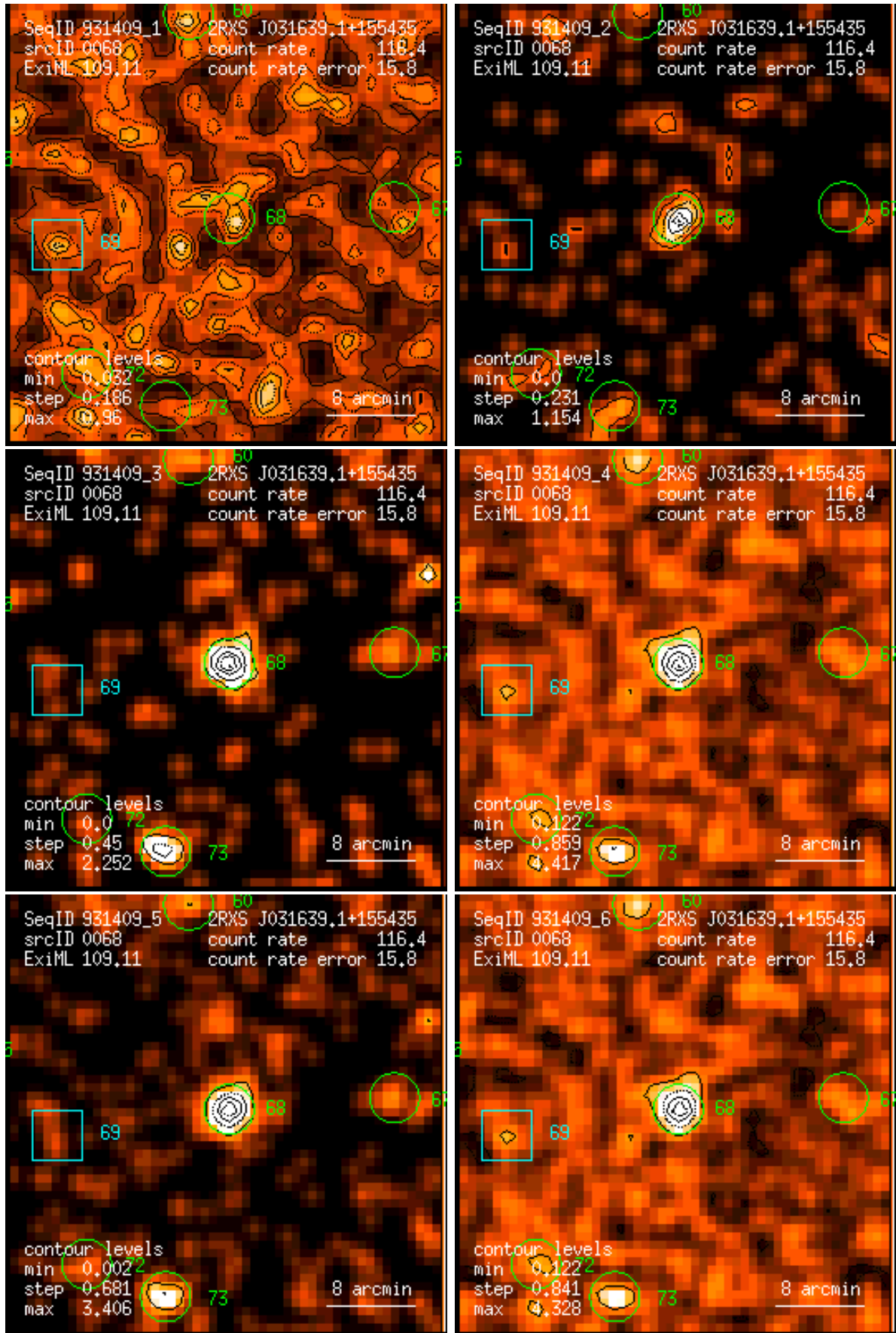
Figure 68: RASS 931409: detection 0068: band rate images, Gaussian filter: (1) PSPC channels 11 – 41, (2) 52 – 90, (3) 91 – 201, (4) 11 – 235, (5) 52 – 201, (6) 11 – 201. Broad band rates in counts/ks. Band rate contour levels in counts/ks/arcmin 2 .
