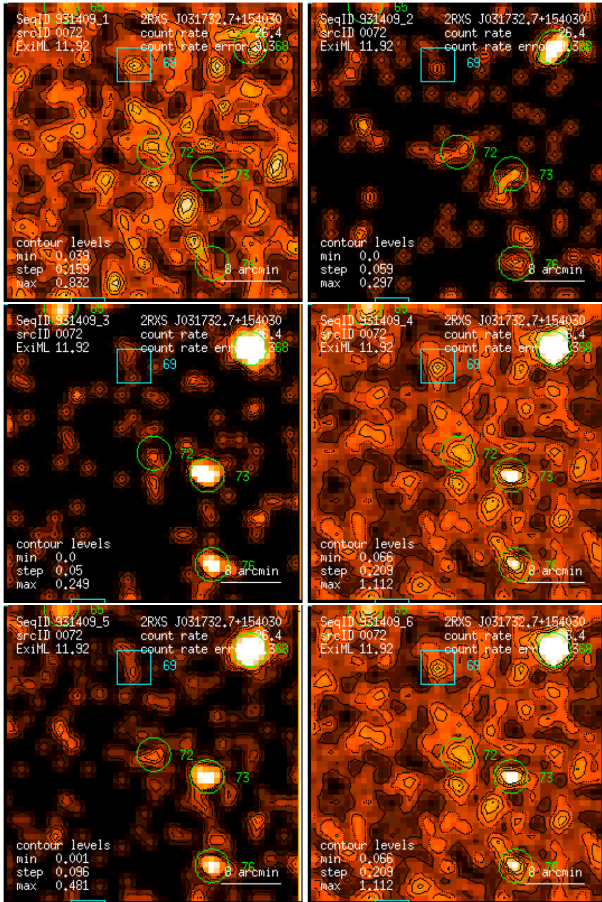
Figure 72: RASS 931409: detection 0072: band rate images, Gaussian filter: (1) PSPC channels 11 – 41, (2) 52 – 90, (3) 91 – 201, (4) 11 – 235, (5) 52 – 201, (6) 11 – 201. Broad band rates in counts/ks. Band rate contour levels in counts/ks/arcmin 2 .
