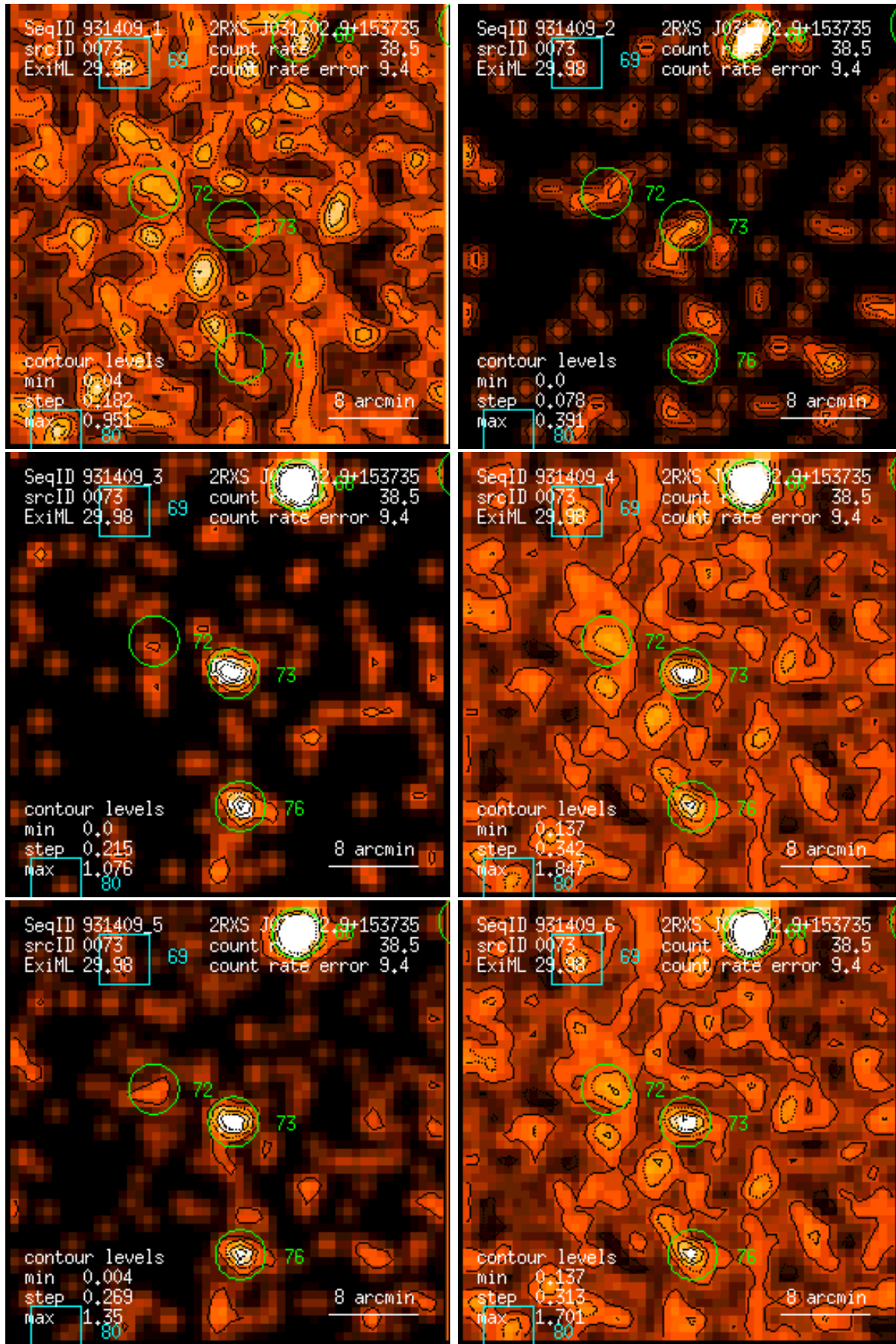
Figure 73: RASS 931409: detection 0073: band rate images, Gaussian filter: (1) PSPC channels 11 – 41, (2) 52 – 90, (3) 91 – 201, (4) 11 – 235, (5) 52 – 201, (6) 11 – 201. Broad band rates in counts/ks. Band rate contour levels in counts/ks/arcmin 2 .
