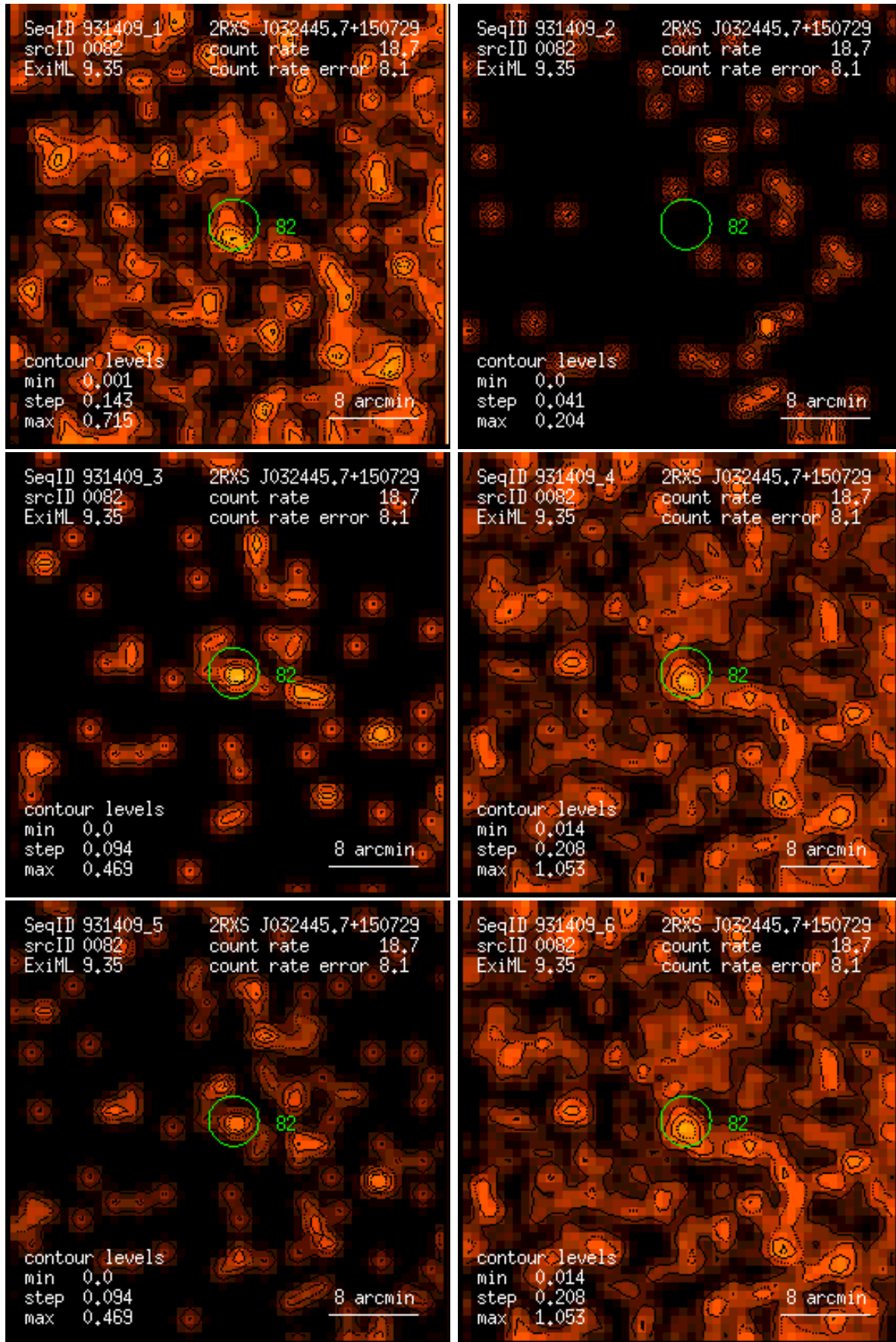
Figure 82: RASS 931409: detection 0082: band rate images, Gaussian filter: (1) PSPC channels 11 – 41, (2) 52 – 90, (3) 91 – 201, (4) 11 – 235, (5) 52 – 201, (6) 11 – 201. Broad band rates in counts/ks. Band rate contour levels in counts/ks/arcmin 2 .
