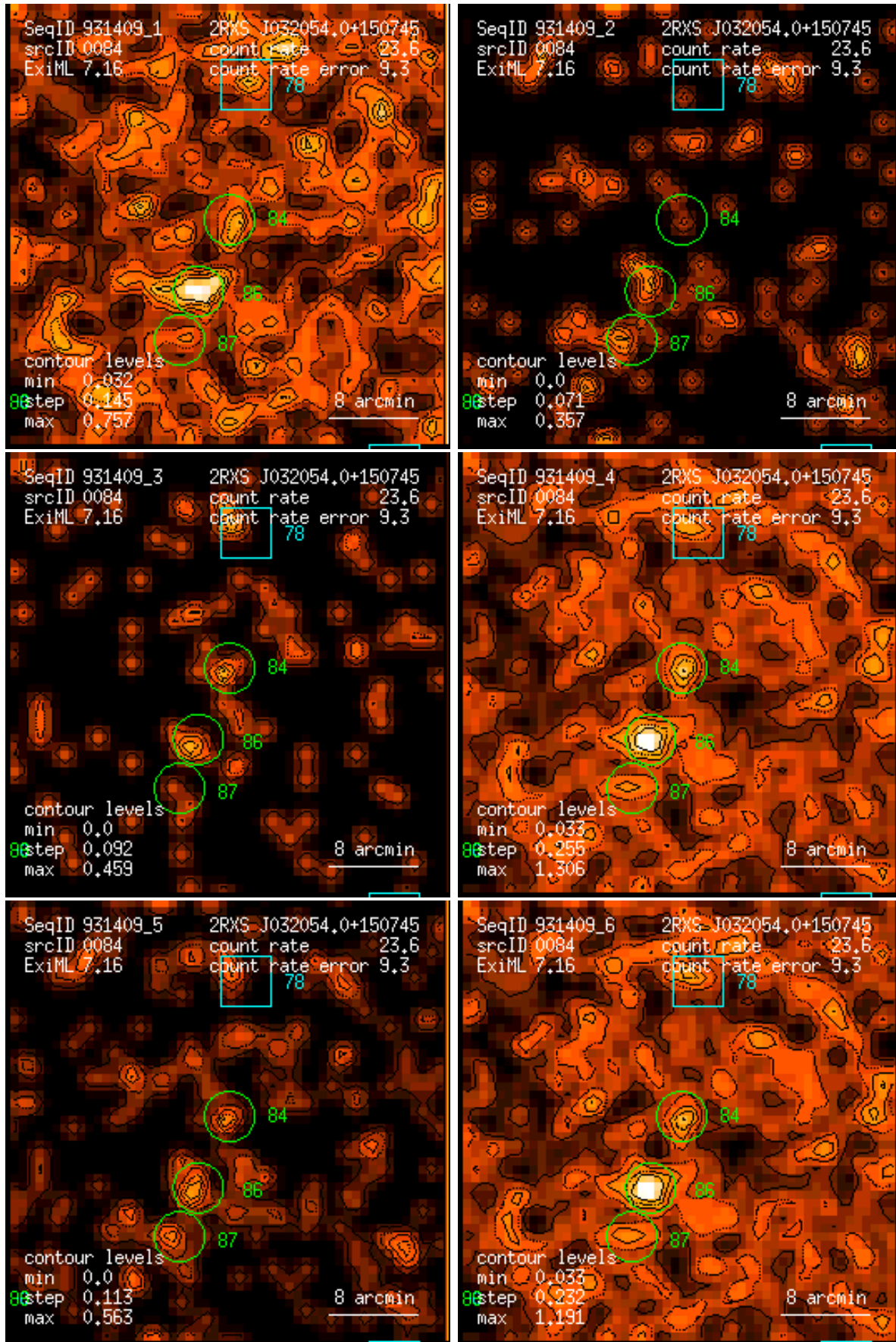
Figure 84: RASS 931409: detection 0084: band rate images, Gaussian filter: (1) PSPC channels 11 – 41, (2) 52 – 90, (3) 91 – 201, (4) 11 – 235, (5) 52 – 201, (6) 11 – 201. Broad band rates in counts/ks. Band rate contour levels in counts/ks/arcmin 2 .
