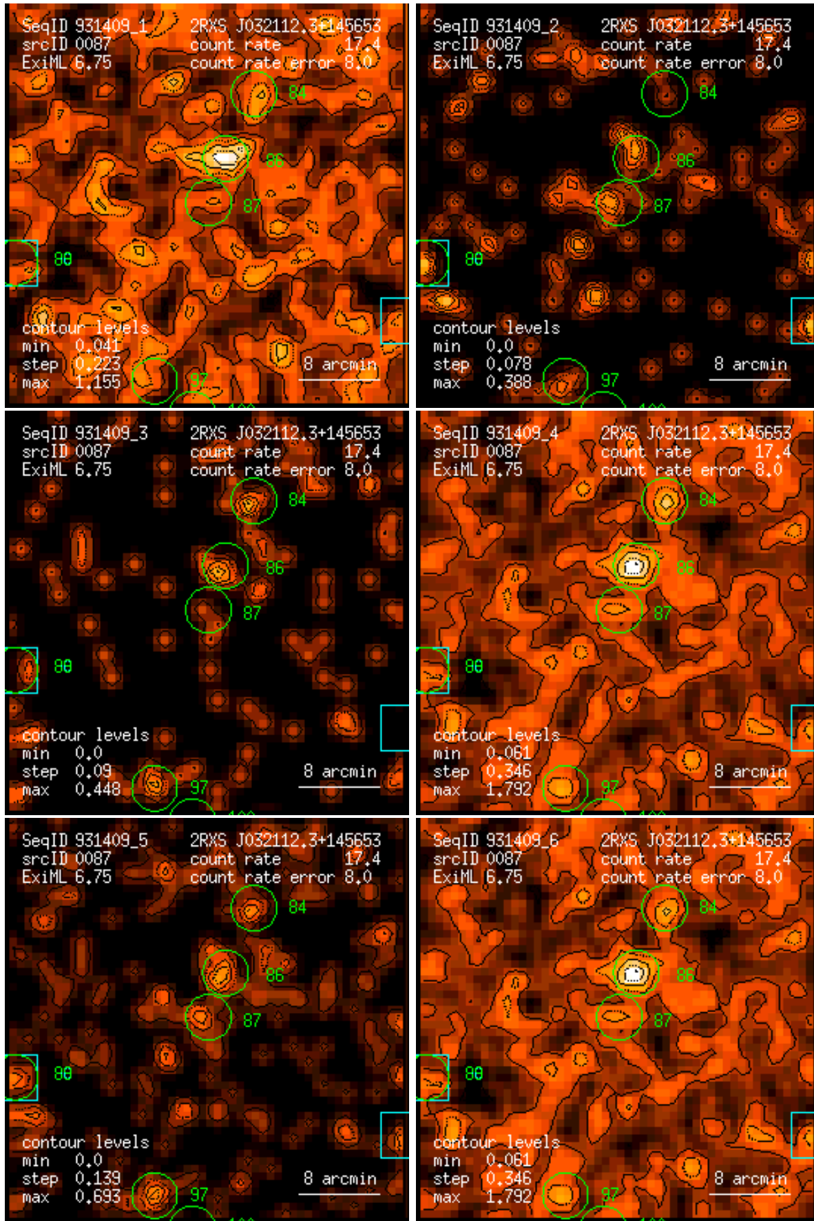
Figure 87: RASS 931409: detection 0087: band rate images, Gaussian filter: (1) PSPC channels 11 – 41, (2) 52 – 90, (3) 91 – 201, (4) 11 – 235, (5) 52 – 201, (6) 11 – 201. Broad band rates in counts/ks. Band rate contour levels in counts/ks/arcmin 2 .
