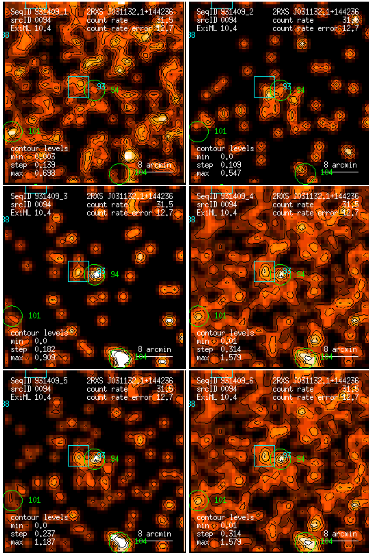
Figure 94: RASS 931409: detection 0094: band rate images, Gaussian filter: (1) PSPC channels 11 – 41, (2) 52 – 90, (3) 91 – 201, (4) 11 – 235, (5) 52 – 201, (6) 11 – 201. Broad band rates in counts/ks. Band rate contour levels in counts/ks/arcmin 2 .
