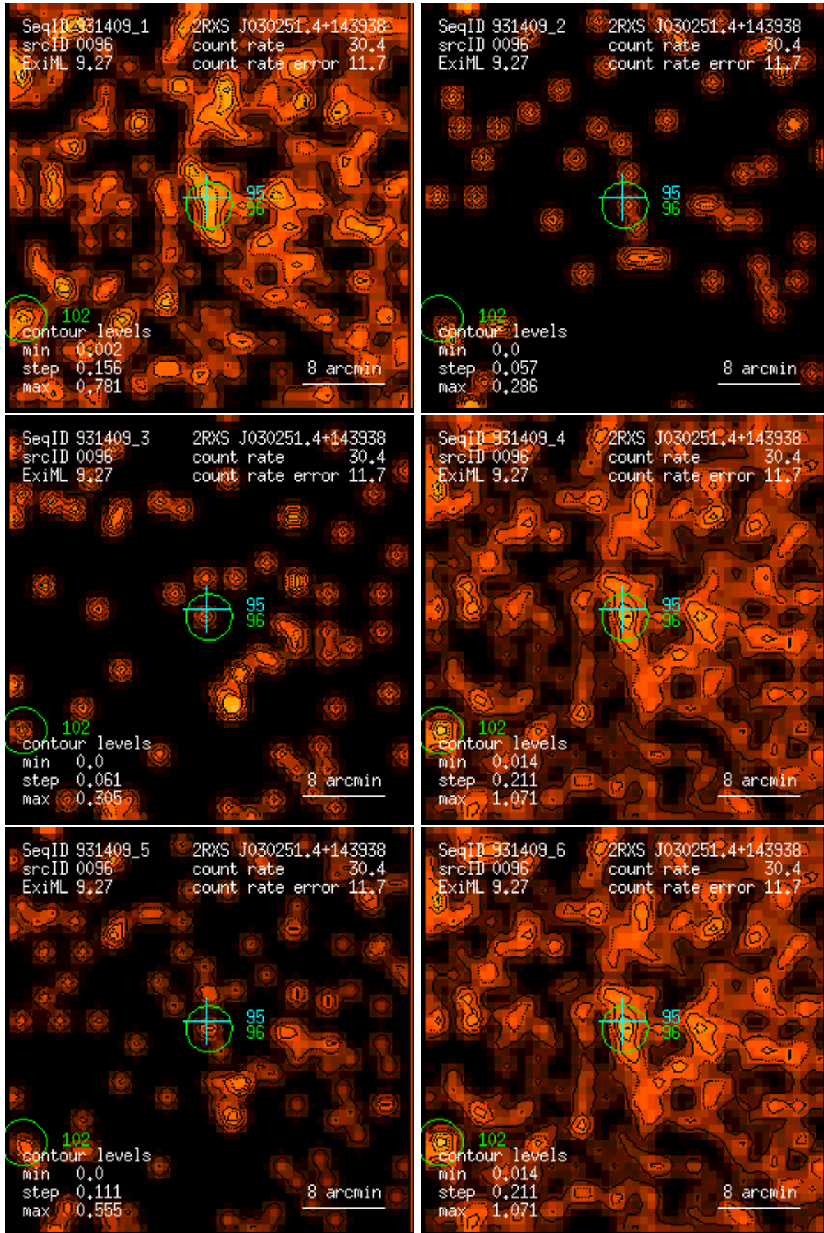
Figure 96: RASS 931409: detection 0096: band rate images, Gaussian filter: (1) PSPC channels 11 – 41, (2) 52 – 90, (3) 91 – 201, (4) 11 – 235, (5) 52 – 201, (6) 11 – 201. Broad band rates in counts/ks. Band rate contour levels in counts/ks/arcmin 2 .
