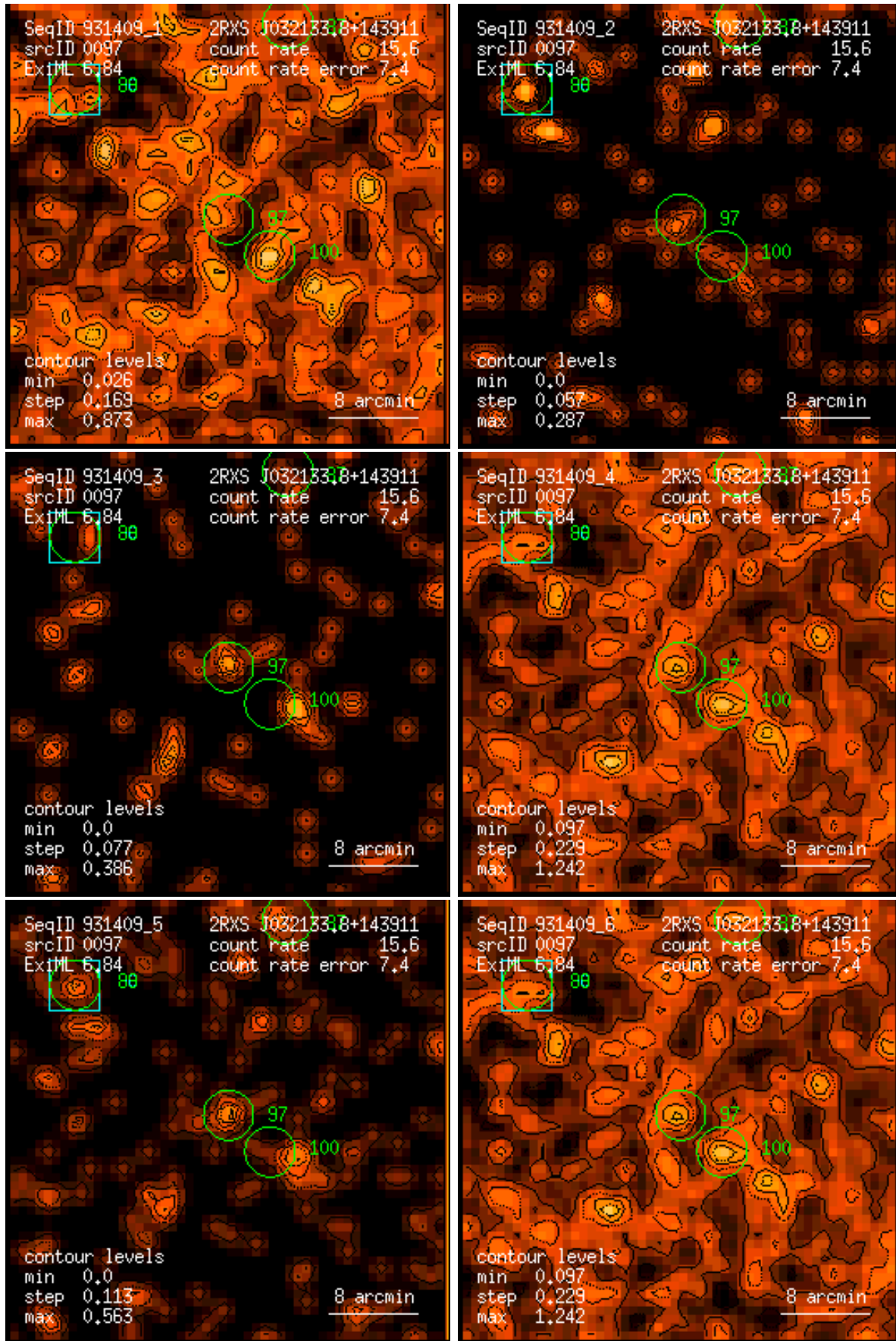
Figure 97: RASS 931409: detection 0097: band rate images, Gaussian filter: (1) PSPC channels 11 – 41, (2) 52 – 90, (3) 91 – 201, (4) 11 – 235, (5) 52 – 201, (6) 11 – 201. Broad band rates in counts/ks. Band rate contour levels in counts/ks/arcmin 2 .
