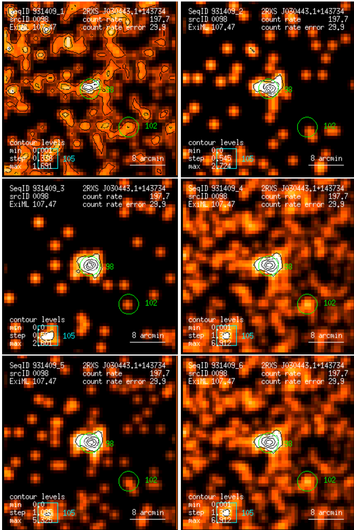
Figure 98: RASS 931409: detection 0098: band rate images, Gaussian filter: (1) PSPC channels 11 – 41, (2) 52 – 90, (3) 91 – 201, (4) 11 – 235, (5) 52 – 201, (6) 11 – 201. Broad band rates in counts/ks. Band rate contour levels in counts/ks/arcmin 2 .
