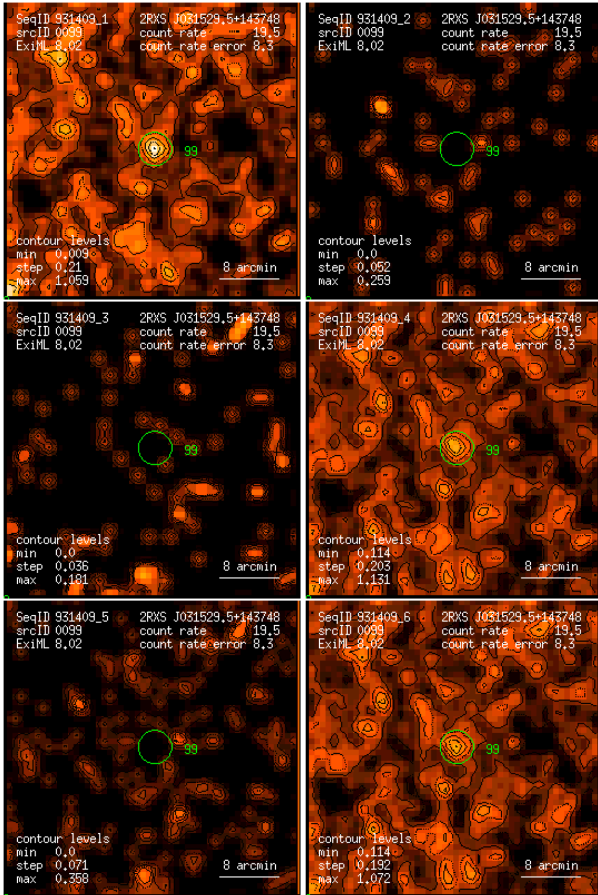
Figure 99: RASS 931409: detection 0099: band rate images, Gaussian filter: (1) PSPC channels 11 – 41, (2) 52 – 90, (3) 91 – 201, (4) 11 – 235, (5) 52 – 201, (6) 11 – 201. Broad band rates in counts/ks. Band rate contour levels in counts/ks/arcmin 2 .
