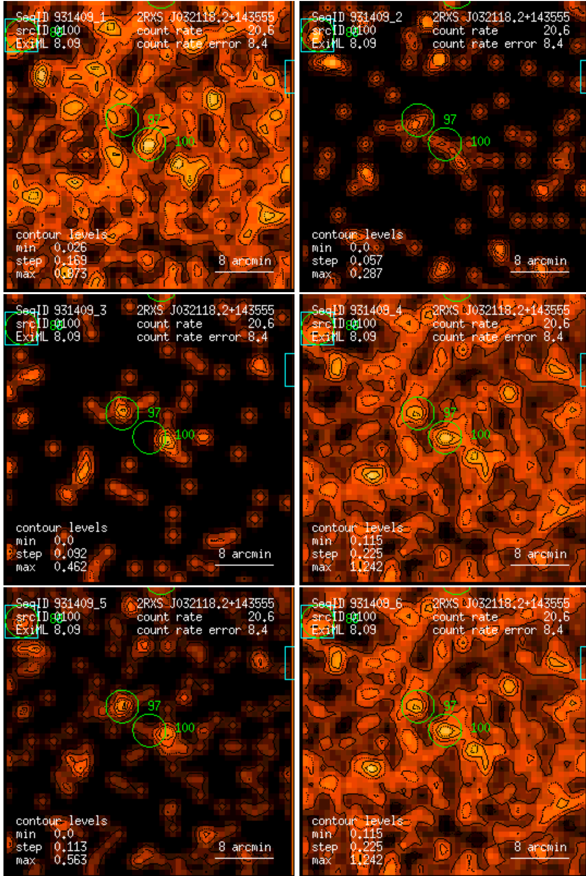
Figure 100: RASS 931409: detection 0100: band rate images, Gaussian filter: (1) PSPC channels 11 – 41, (2) 52 – 90, (3) 91 – 201, (4) 11 – 235, (5) 52 – 201, (6) 11 – 201. Broad band rates in counts/ks. Band rate contour levels in counts/ks/arcmin 2 .
