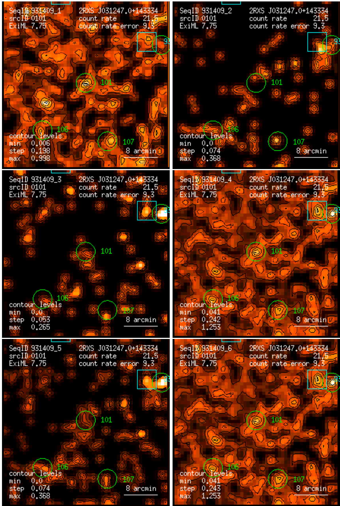
Figure 101: RASS 931409: detection 0101: band rate images, Gaussian filter: (1) PSPC channels 11 – 41, (2) 52 – 90, (3) 91 – 201, (4) 11 – 235, (5) 52 – 201, (6) 11 – 201. Broad band rates in counts/ks. Band rate contour levels in counts/ks/arcmin 2 .
