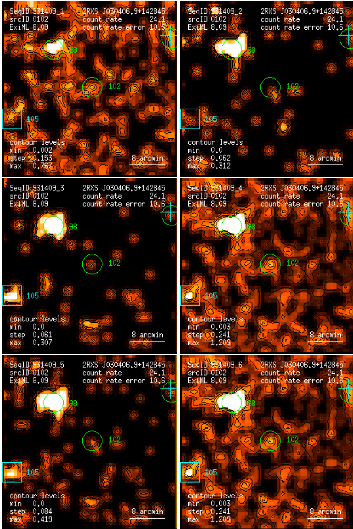
Figure 102: RASS 931409: detection 0102: band rate images, Gaussian filter: (1) PSPC channels 11 – 41, (2) 52 – 90, (3) 91 – 201, (4) 11 – 235, (5) 52 – 201, (6) 11 – 201. Broad band rates in counts/ks. Band rate contour levels in counts/ks/arcmin 2 .
