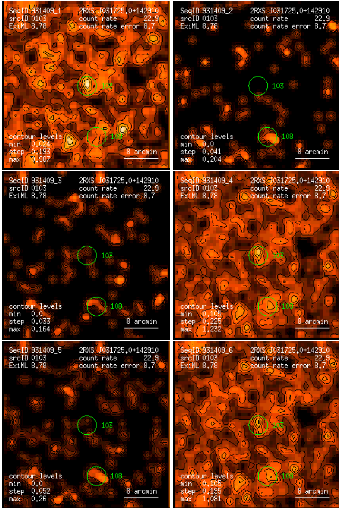
Figure 103: RASS 931409: detection 0103: band rate images, Gaussian filter: (1) PSPC channels 11 – 41, (2) 52 – 90, (3) 91 – 201, (4) 11 – 235, (5) 52 – 201, (6) 11 – 201. Broad band rates in counts/ks. Band rate contour levels in counts/ks/arcmin 2 .
