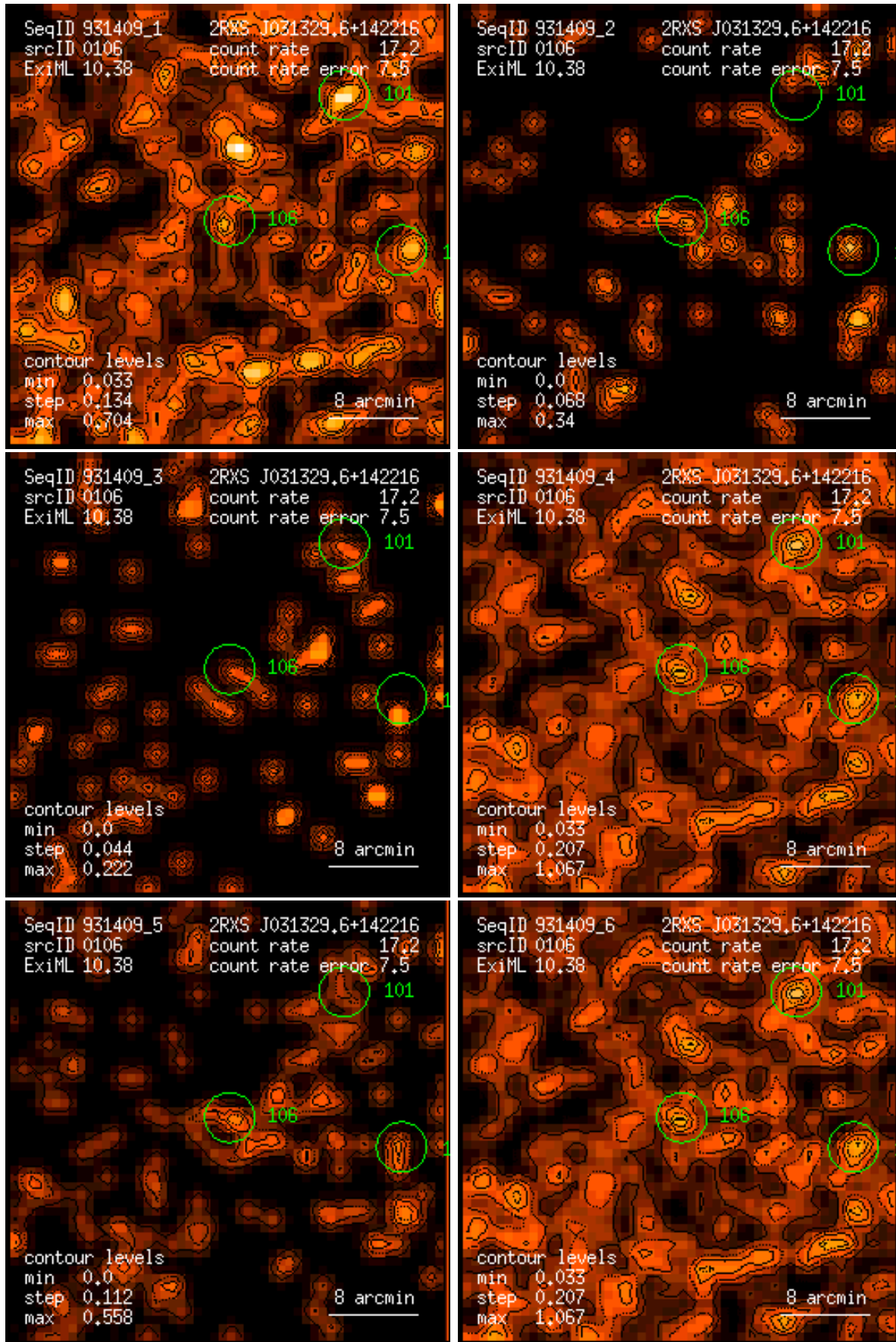
Figure 106: RASS 931409: detection 0106: band rate images, Gaussian filter: (1) PSPC channels 11 – 41, (2) 52 – 90, (3) 91 – 201, (4) 11 – 235, (5) 52 – 201, (6) 11 – 201. Broad band rates in counts/ks. Band rate contour levels in counts/ks/arcmin 2 .
