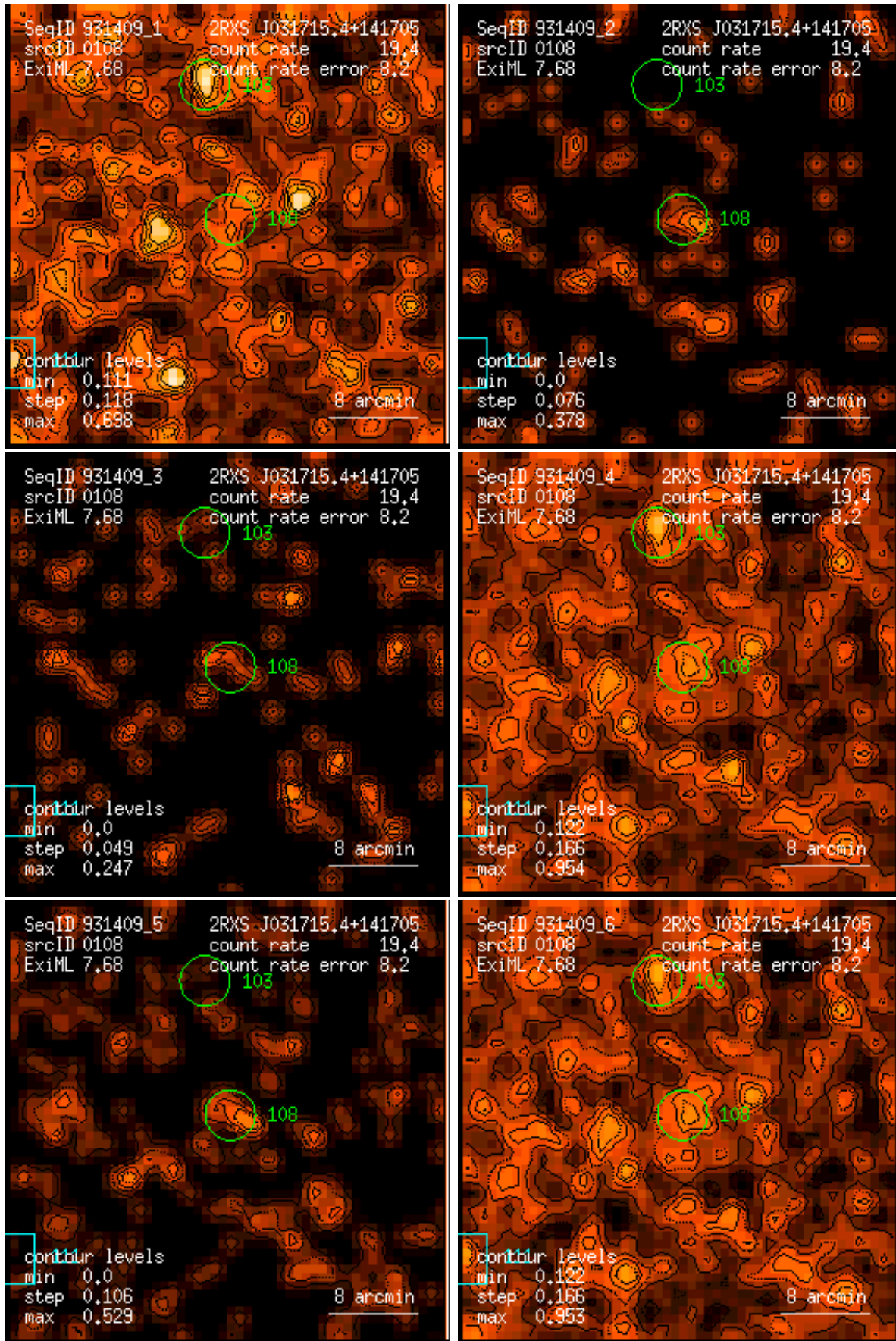
Figure 108: RASS 931409: detection 0108: band rate images, Gaussian filter: (1) PSPC channels 11 – 41, (2) 52 – 90, (3) 91 – 201, (4) 11 – 235, (5) 52 – 201, (6) 11 – 201. Broad band rates in counts/ks. Band rate contour levels in counts/ks/arcmin 2 .
