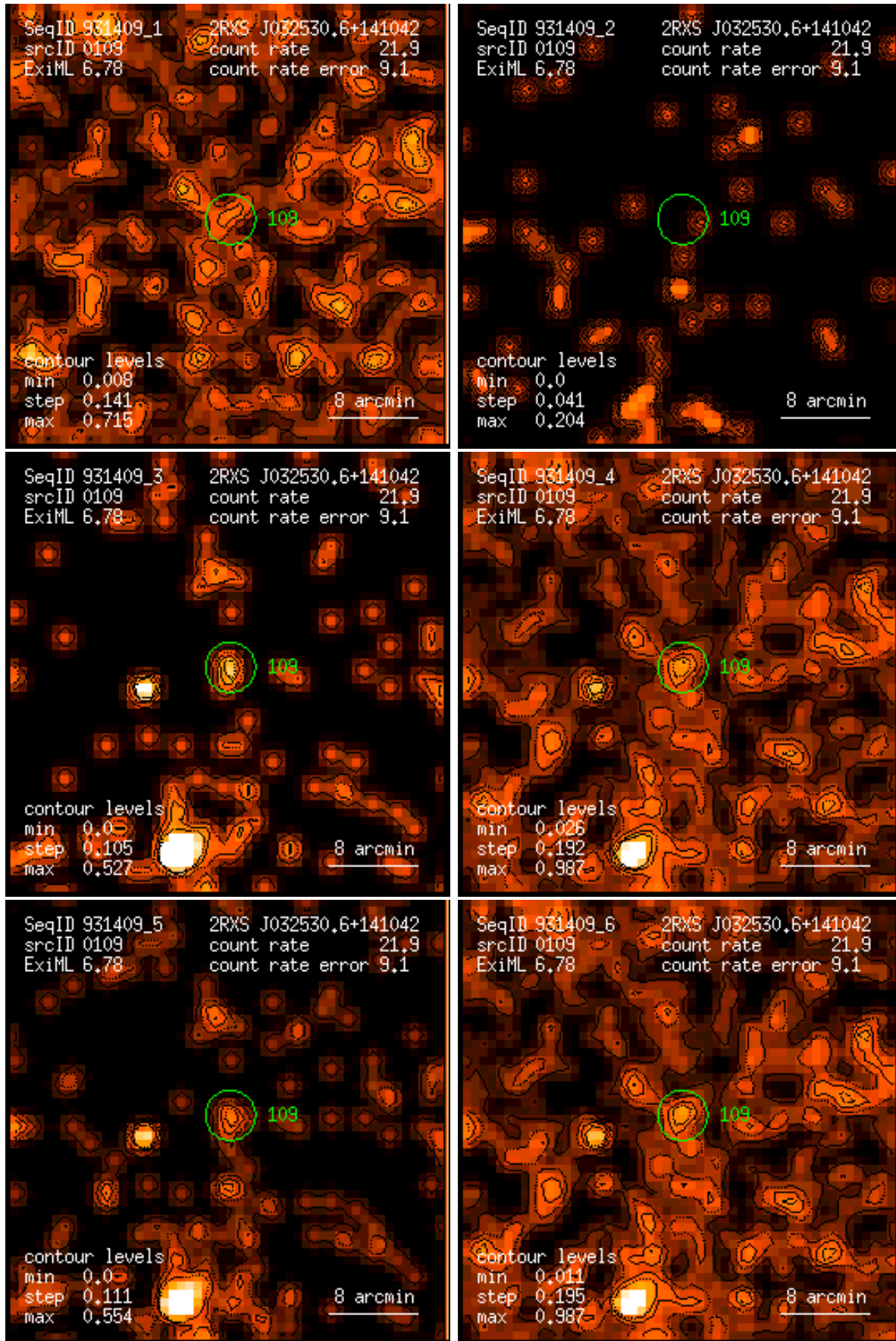
Figure 109: RASS 931409: detection 0109: band rate images, Gaussian filter: (1) PSPC channels 11 – 41, (2) 52 – 90, (3) 91 – 201, (4) 11 – 235, (5) 52 – 201, (6) 11 – 201. Broad band rates in counts/ks. Band rate contour levels in counts/ks/arcmin 2 .
