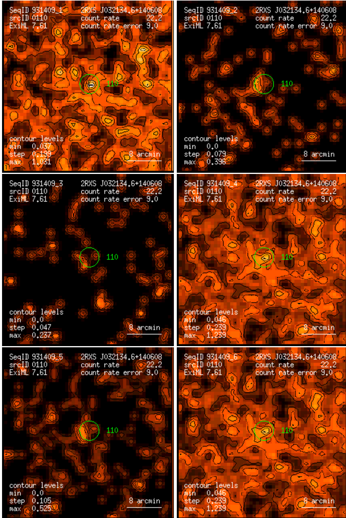
Figure 110: RASS 931409: detection 0110: band rate images, Gaussian filter: (1) PSPC channels 11 – 41, (2) 52 – 90, (3) 91 – 201, (4) 11 – 235, (5) 52 – 201, (6) 11 – 201. Broad band rates in counts/ks. Band rate contour levels in counts/ks/arcmin 2 .
