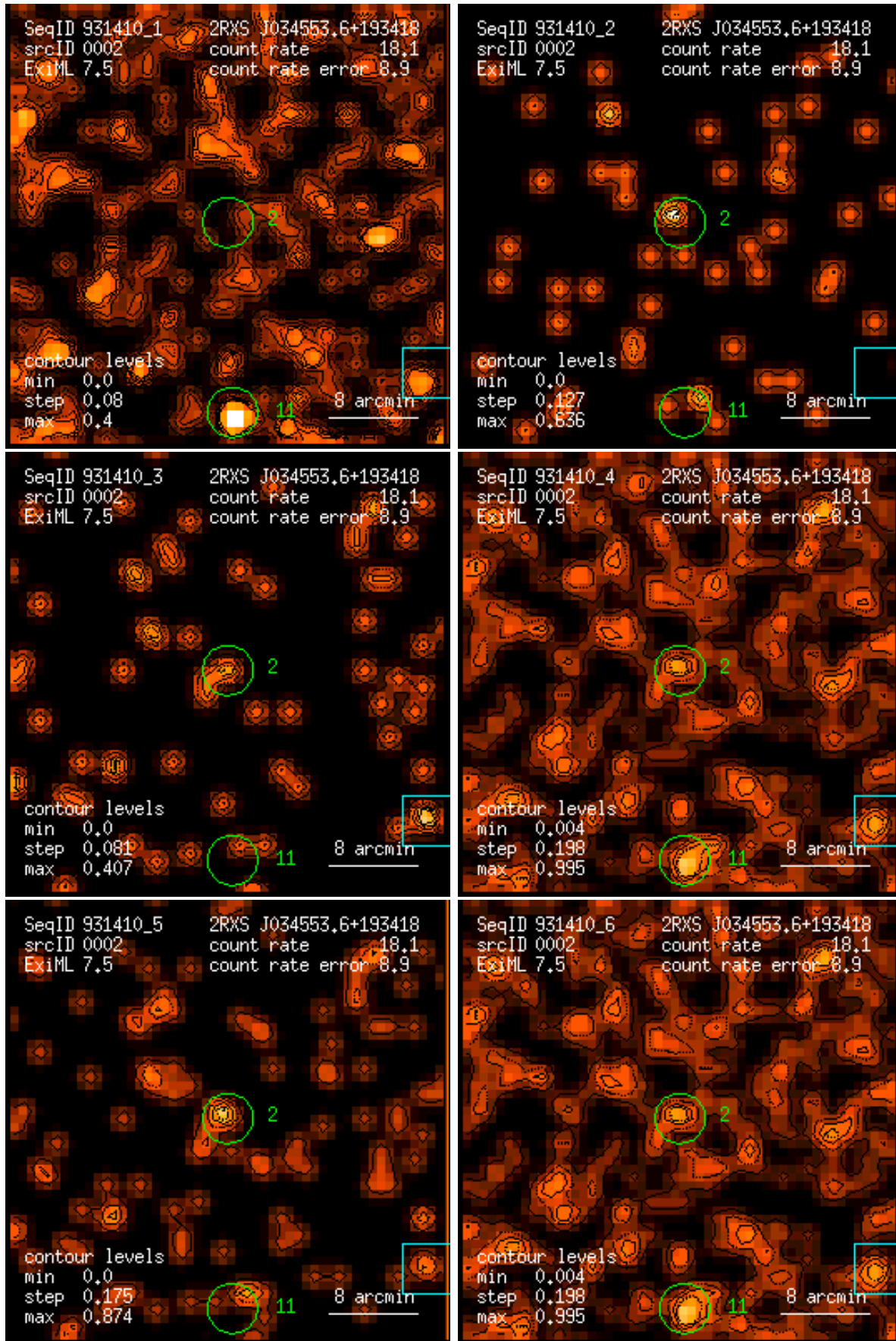
Figure 2: RASS 931410: detection 0002: band rate images, Gaussian filter: (1) PSPC channels 11 – 41, (2) 52 – 90, (3) 91 – 201, (4) 11 – 235, (5) 52 – 201, (6) 11 – 201. Broad band rates in counts/ks. Band rate contour levels in counts/ks/arcmin 2 .
