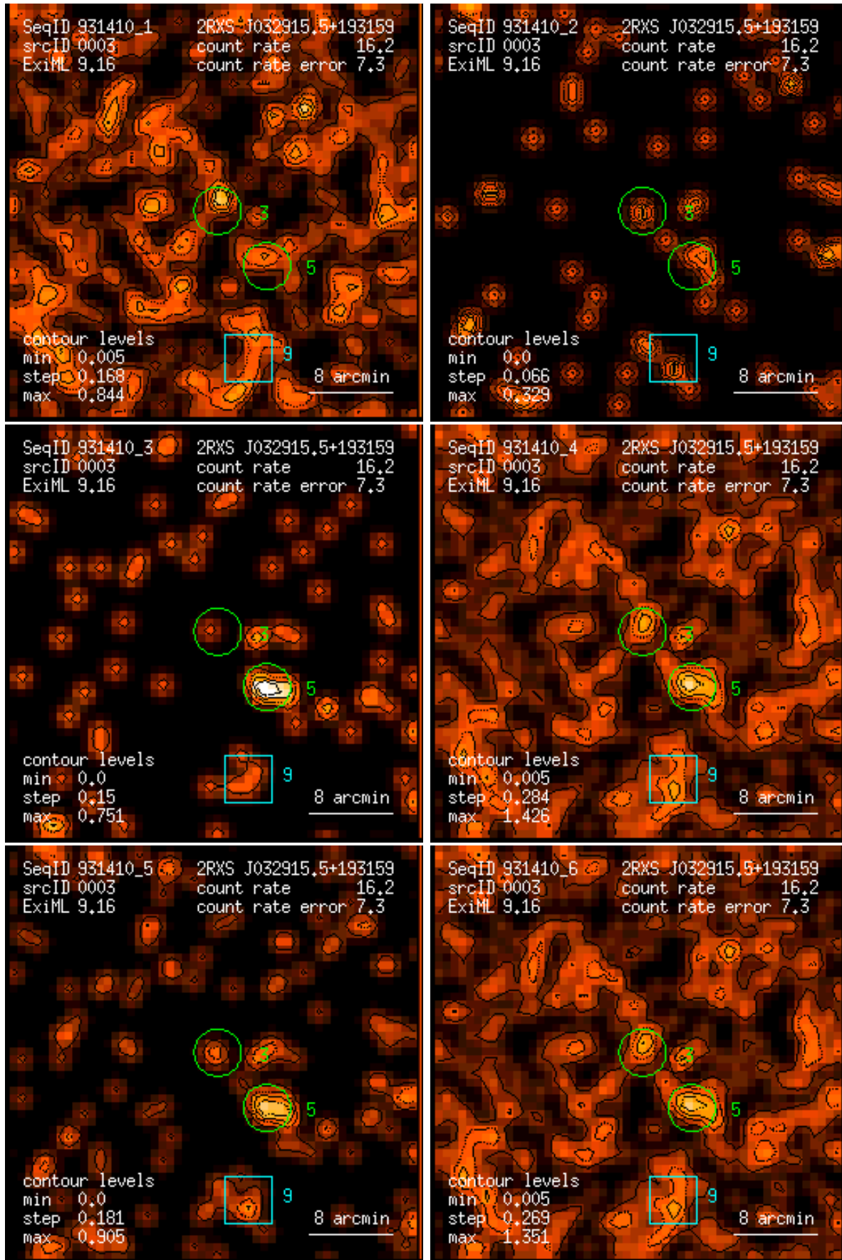
Figure 3: RASS 931410: detection 0003: band rate images, Gaussian filter: (1) PSPC channels 11 – 41, (2) 52 – 90, (3) 91 – 201, (4) 11 – 235, (5) 52 – 201, (6) 11 – 201. Broad band rates in counts/ks. Band rate contour levels in counts/ks/arcmin 2 .
