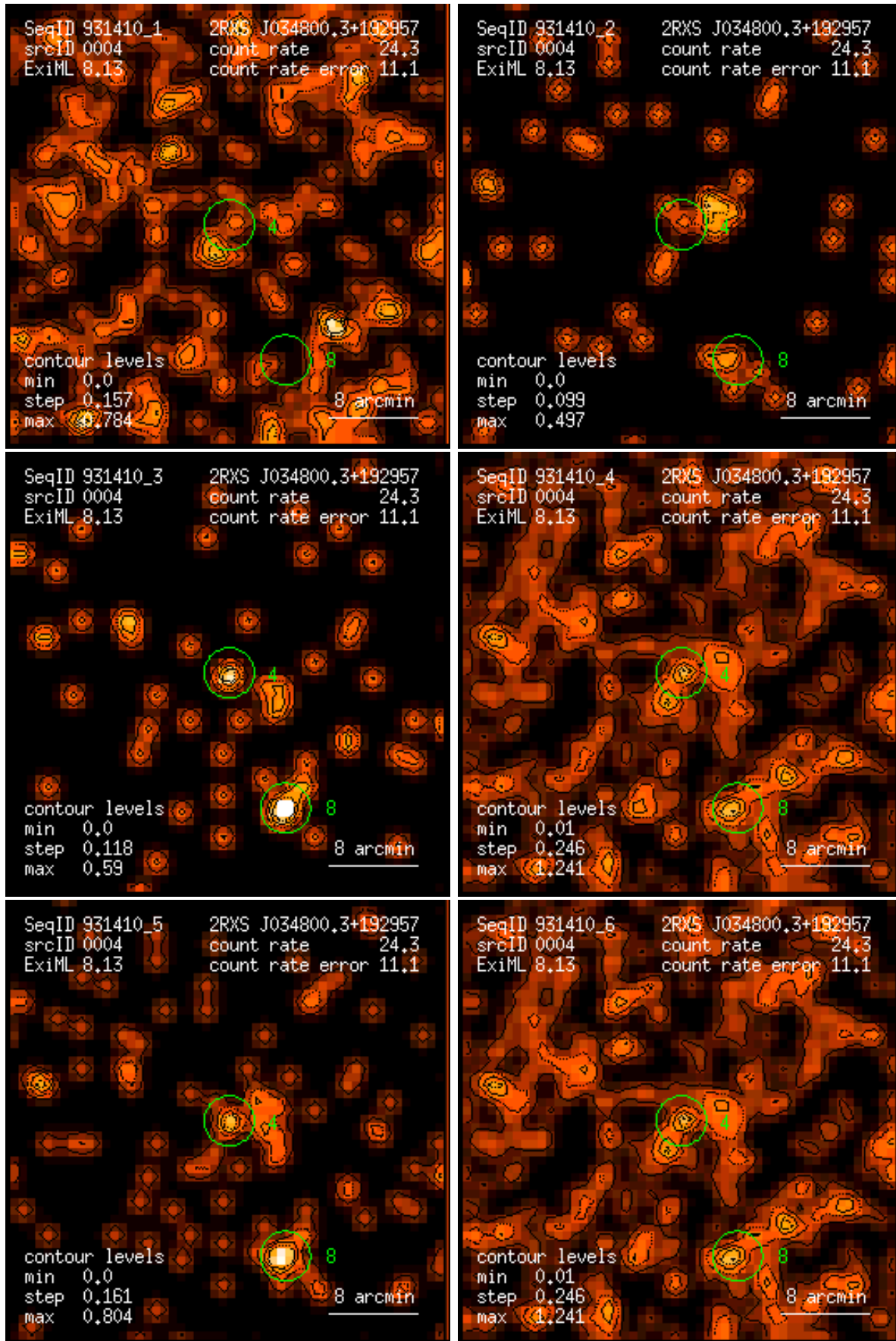
Figure 4: RASS 931410: detection 0004: band rate images, Gaussian filter: (1) PSPC channels 11 – 41, (2) 52 – 90, (3) 91 – 201, (4) 11 – 235, (5) 52 – 201, (6) 11 – 201. Broad band rates in counts/ks. Band rate contour levels in counts/ks/arcmin 2 .
