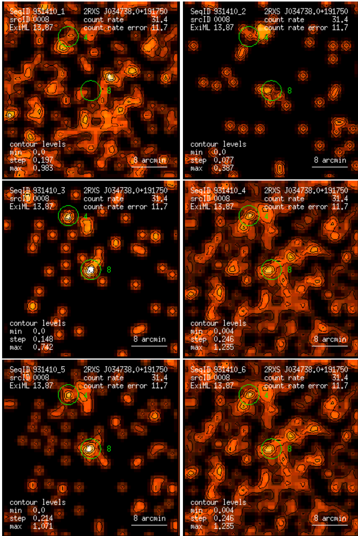
Figure 8: RASS 931410: detection 0008: band rate images, Gaussian filter: (1) PSPC channels 11 – 41, (2) 52 – 90, (3) 91 – 201, (4) 11 – 235, (5) 52 – 201, (6) 11 – 201. Broad band rates in counts/ks. Band rate contour levels in counts/ks/arcmin 2 .
