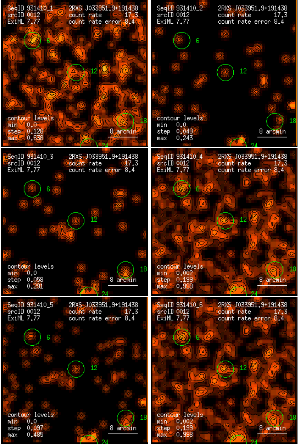
Figure 12: RASS 931410: detection 0012: band rate images, Gaussian filter: (1) PSPC channels 11 – 41, (2) 52 – 90, (3) 91 – 201, (4) 11 – 235, (5) 52 – 201, (6) 11 – 201. Broad band rates in counts/ks. Band rate contour levels in counts/ks/arcmin 2 .
