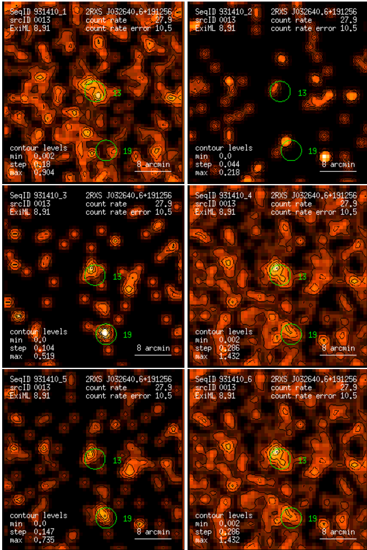
Figure 13: RASS 931410: detection 0013: band rate images, Gaussian filter: (1) PSPC channels 11 – 41, (2) 52 – 90, (3) 91 – 201, (4) 11 – 235, (5) 52 – 201, (6) 11 – 201. Broad band rates in counts/ks. Band rate contour levels in counts/ks/arcmin 2 .
