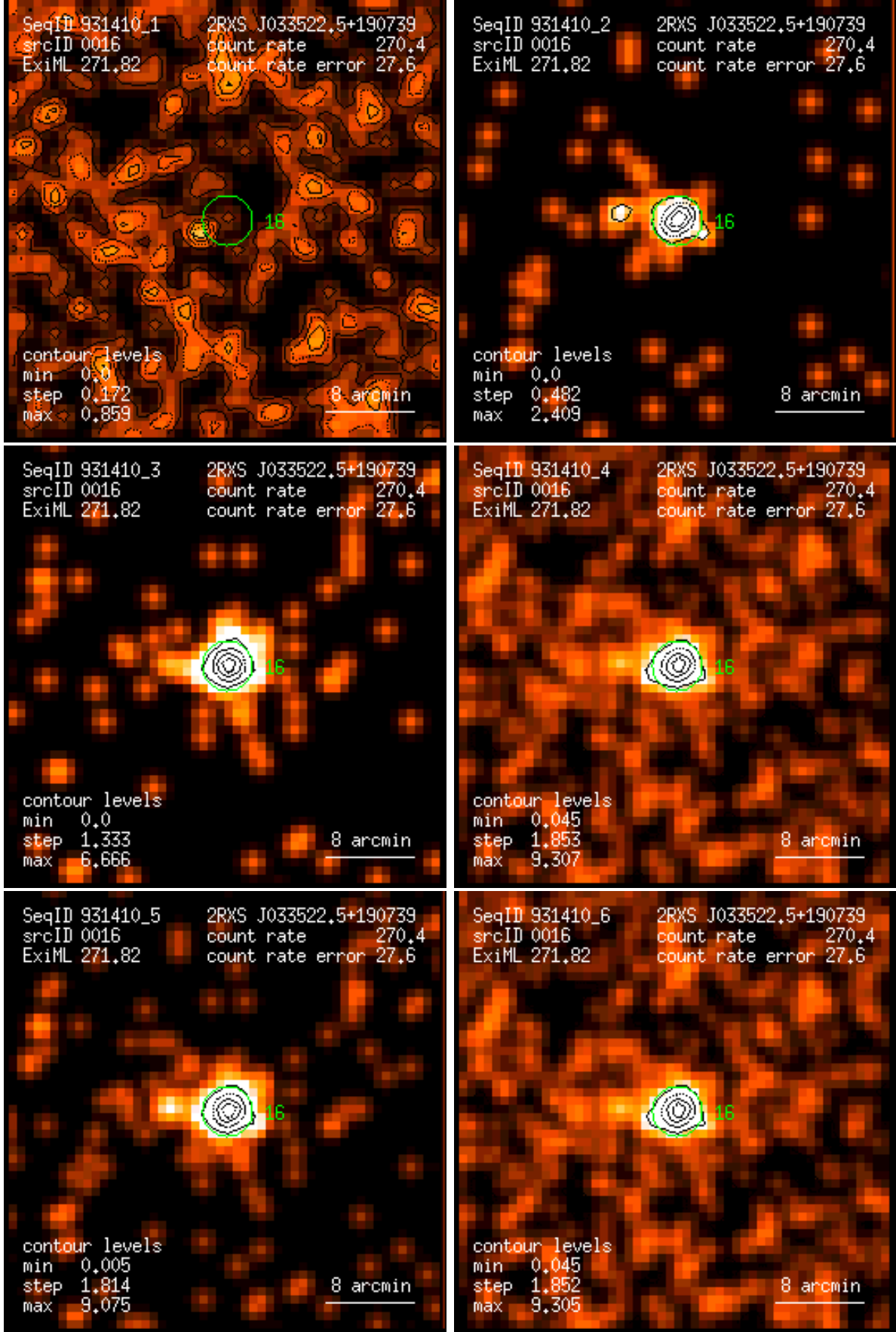
Figure 16: RASS 931410: detection 0016: band rate images, Gaussian filter: (1) PSPC channels 11 – 41, (2) 52 – 90, (3) 91 – 201, (4) 11 – 235, (5) 52 – 201, (6) 11 – 201. Broad band rates in counts/ks. Band rate contour levels in counts/ks/arcmin 2 .
